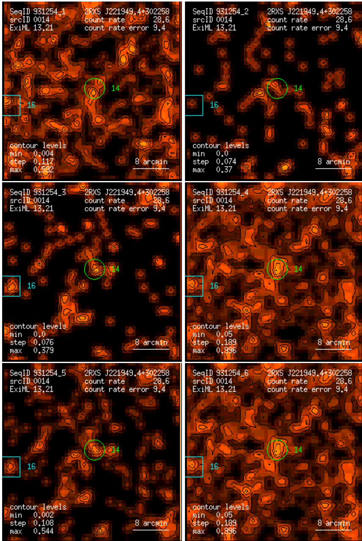
Figure 14: RASS 931254: detection 0014: band rate images, Gaussian filter: (1) PSPC channels 11 – 41, (2) 52 – 90, (3) 91 – 201, (4) 11 – 235, (5) 52 – 201, (6) 11 – 201. Broad band rates in counts/ks. Band rate contour levels in counts/ks/arcmin 2 .
