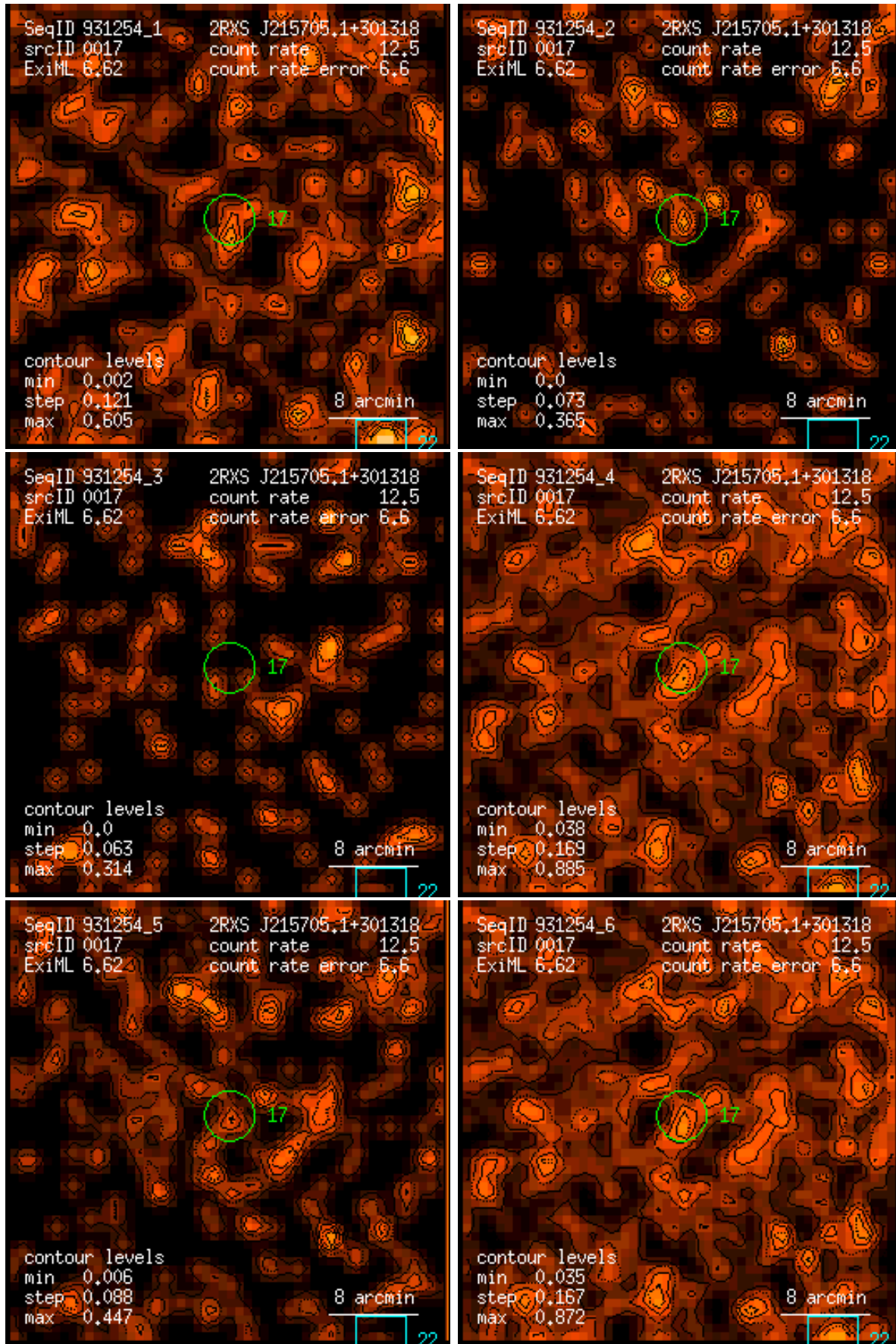
Figure 17: RASS 931254: detection 0017: band rate images, Gaussian filter: (1) PSPC channels 11 – 41, (2) 52 – 90, (3) 91 – 201, (4) 11 – 235, (5) 52 – 201, (6) 11 – 201. Broad band rates in counts/ks. Band rate contour levels in counts/ks/arcmin 2 .
