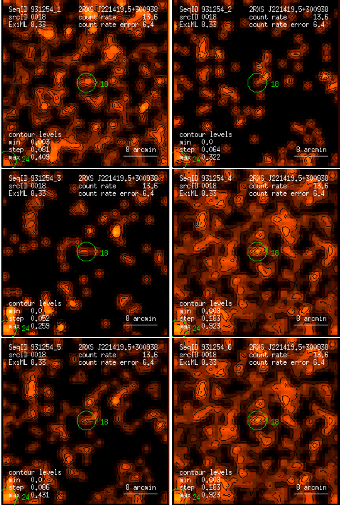
Figure 18: RASS 931254: detection 0018: band rate images, Gaussian filter: (1) PSPC channels 11 – 41, (2) 52 – 90, (3) 91 – 201, (4) 11 – 235, (5) 52 – 201, (6) 11 – 201. Broad band rates in counts/ks. Band rate contour levels in counts/ks/arcmin 2 .
