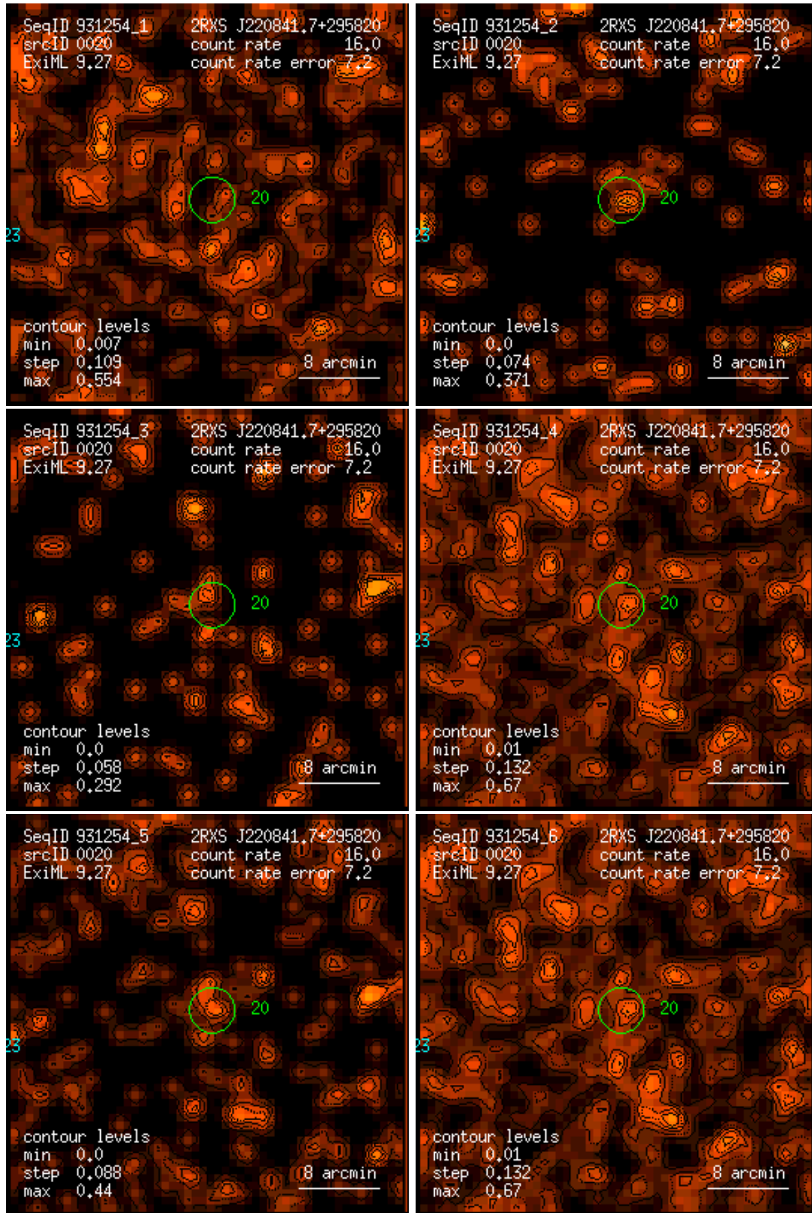
Figure 20: RASS 931254: detection 0020: band rate images, Gaussian filter: (1) PSPC channels 11 – 41, (2) 52 – 90, (3) 91 – 201, (4) 11 – 235, (5) 52 – 201, (6) 11 – 201. Broad band rates in counts/ks. Band rate contour levels in counts/ks/arcmin 2 .
