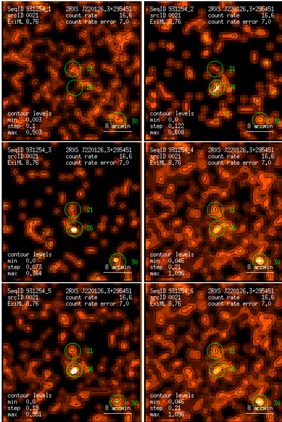
Figure 21: RASS 931254: detection 0021: band rate images, Gaussian filter: (1) PSPC channels 11 – 41, (2) 52 – 90, (3) 91 – 201, (4) 11 – 235, (5) 52 – 201, (6) 11 – 201. Broad band rates in counts/ks. Band rate contour levels in counts/ks/arcmin 2 .
