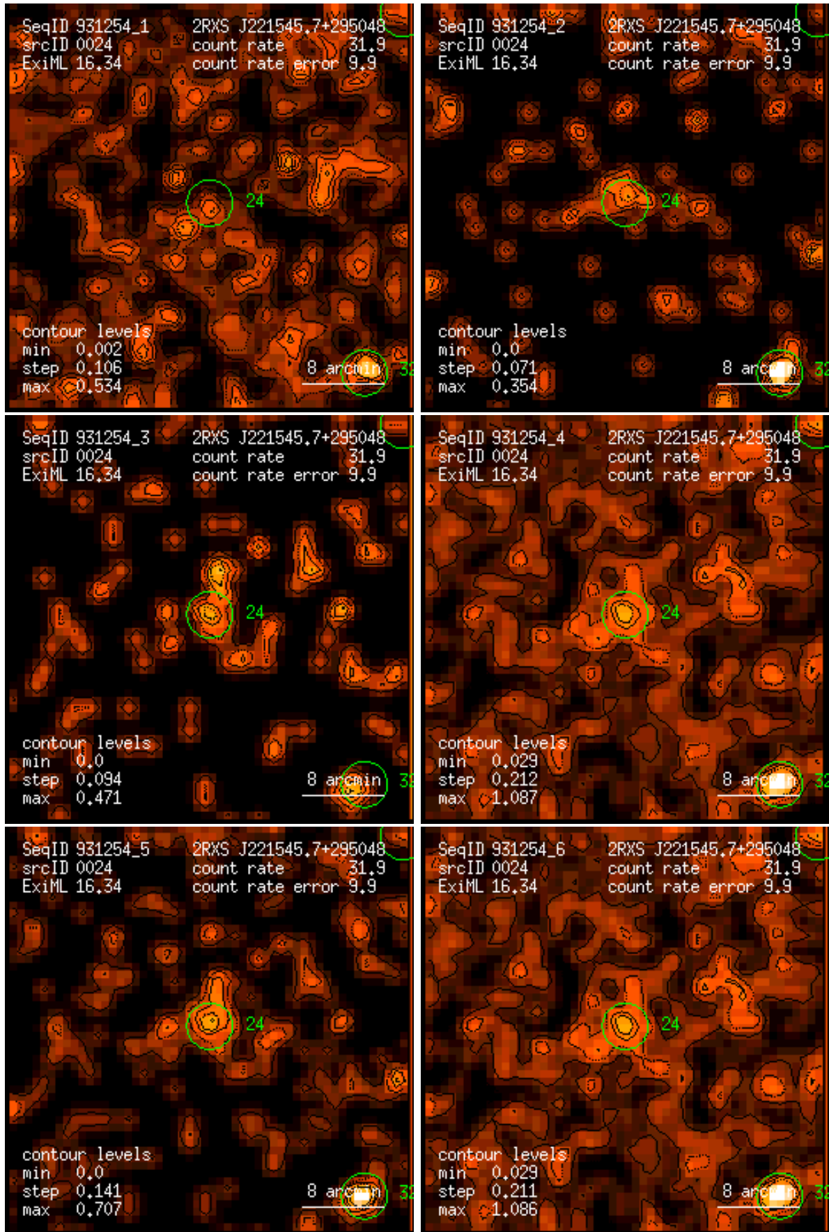
Figure 24: RASS 931254: detection 0024: band rate images, Gaussian filter: (1) PSPC channels 11 – 41, (2) 52 – 90, (3) 91 – 201, (4) 11 – 235, (5) 52 – 201, (6) 11 – 201. Broad band rates in counts/ks. Band rate contour levels in counts/ks/arcmin 2 .
