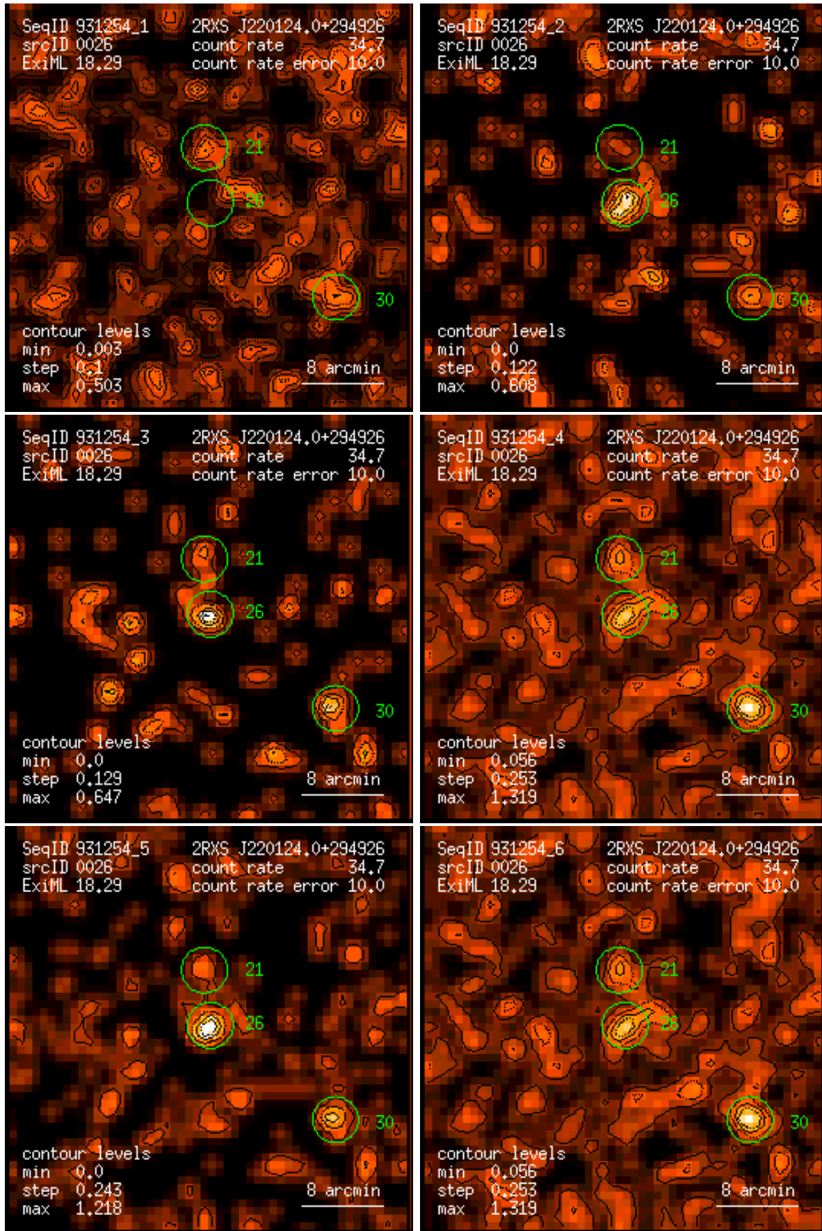
Figure 26: RASS 931254: detection 0026: band rate images, Gaussian filter: (1) PSPC channels 11 – 41, (2) 52 – 90, (3) 91 – 201, (4) 11 – 235, (5) 52 – 201, (6) 11 – 201. Broad band rates in counts/ks. Band rate contour levels in counts/ks/arcmin 2 .
