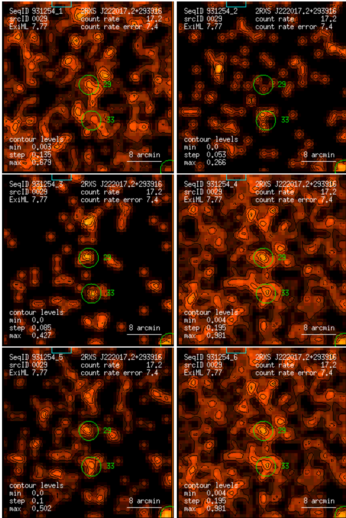
Figure 29: RASS 931254: detection 0029: band rate images, Gaussian filter: (1) PSPC channels 11 – 41, (2) 52 – 90, (3) 91 – 201, (4) 11 – 235, (5) 52 – 201, (6) 11 – 201. Broad band rates in counts/ks. Band rate contour levels in counts/ks/arcmin 2 .
