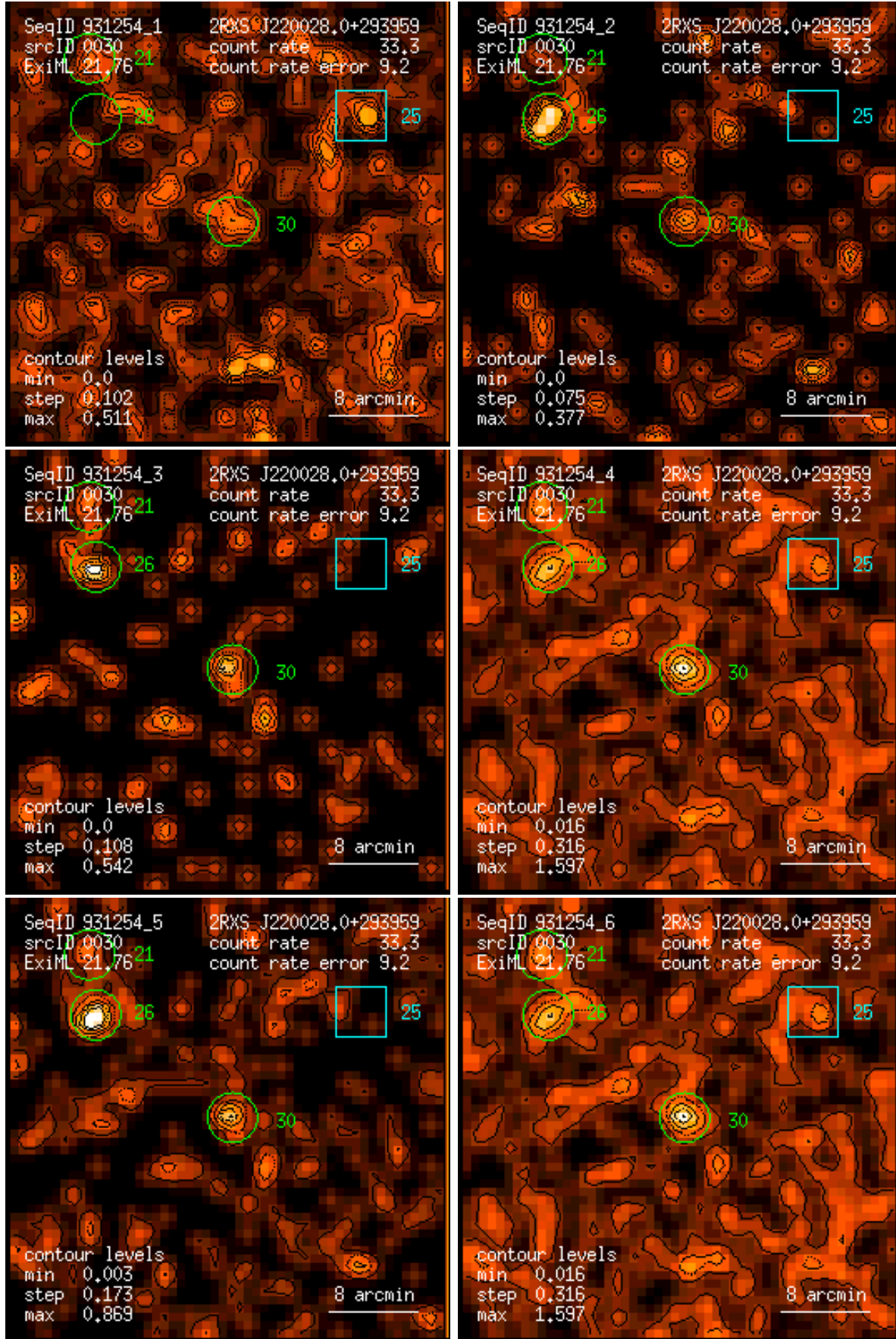
Figure 30: RASS 931254: detection 0030: band rate images, Gaussian filter: (1) PSPC channels 11 – 41, (2) 52 – 90, (3) 91 – 201, (4) 11 – 235, (5) 52 – 201, (6) 11 – 201. Broad band rates in counts/ks. Band rate contour levels in counts/ks/arcmin 2 .
