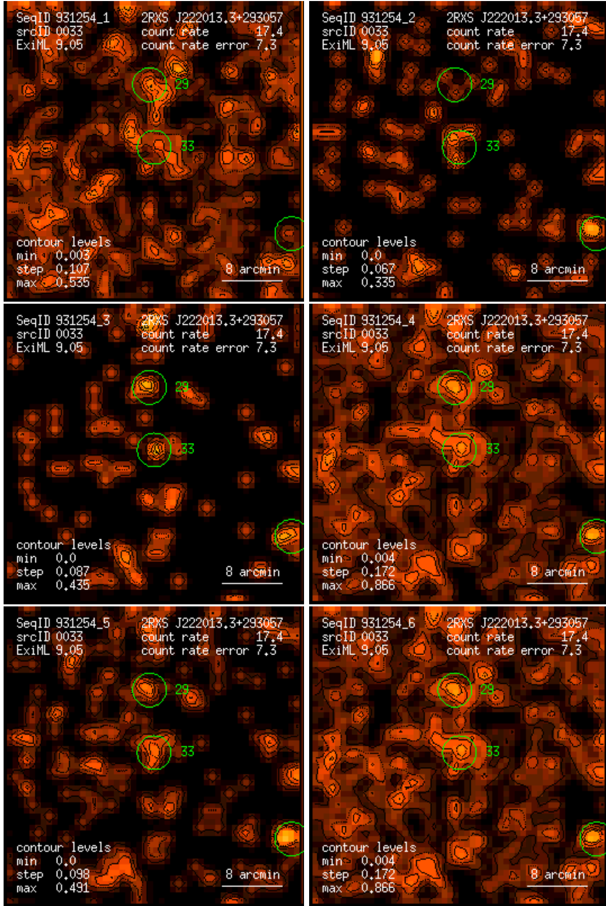
Figure 33: RASS 931254: detection 0033: band rate images, Gaussian filter: (1) PSPC channels 11 – 41, (2) 52 – 90, (3) 91 – 201, (4) 11 – 235, (5) 52 – 201, (6) 11 – 201. Broad band rates in counts/ks. Band rate contour levels in counts/ks/arcmin 2 .
