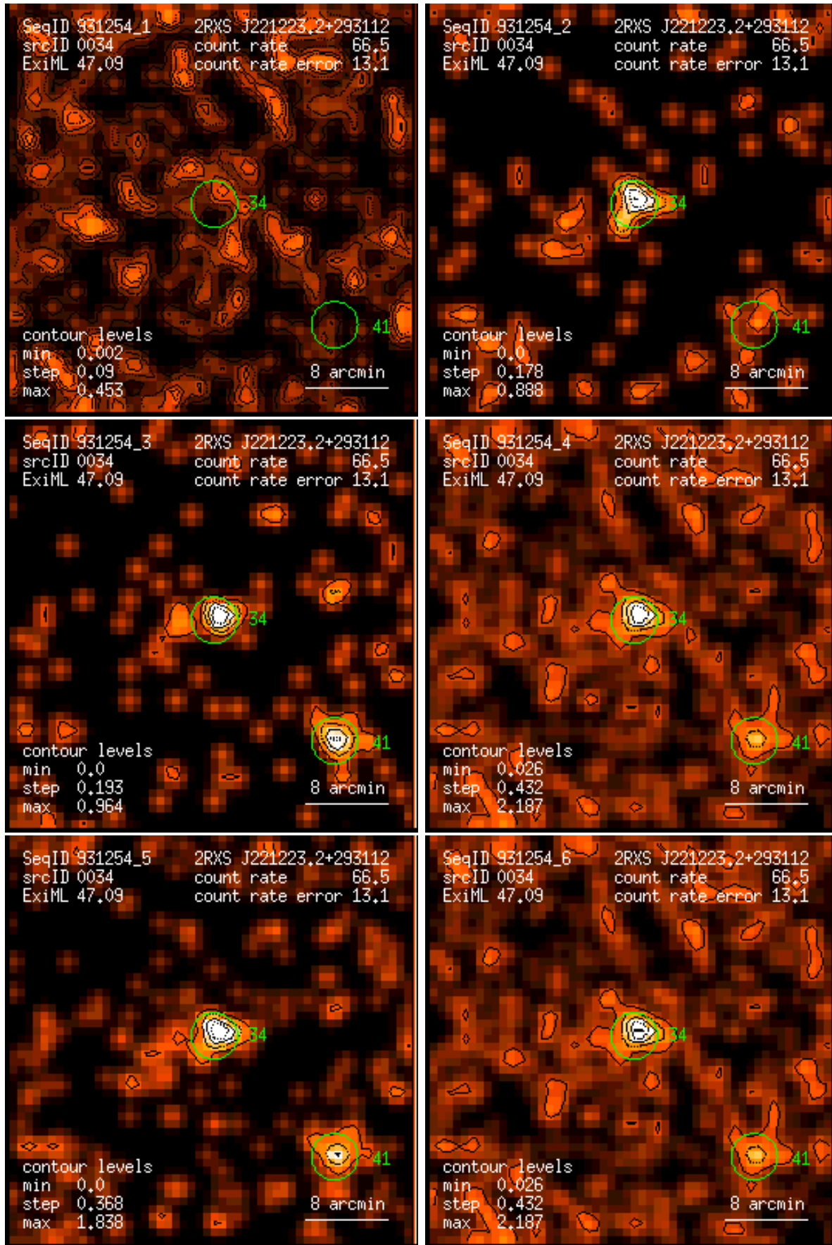
Figure 34: RASS 931254: detection 0034: band rate images, Gaussian filter: (1) PSPC channels 11 – 41, (2) 52 – 90, (3) 91 – 201, (4) 11 – 235, (5) 52 – 201, (6) 11 – 201. Broad band rates in counts/ks. Band rate contour levels in counts/ks/arcmin 2 .
