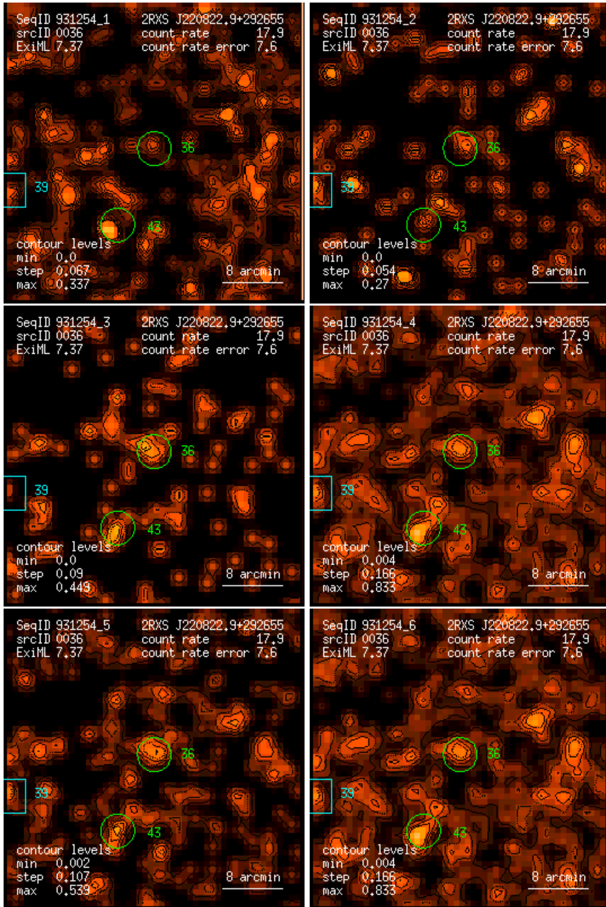
Figure 36: RASS 931254: detection 0036: band rate images, Gaussian filter: (1) PSPC channels 11 – 41, (2) 52 – 90, (3) 91 – 201, (4) 11 – 235, (5) 52 – 201, (6) 11 – 201. Broad band rates in counts/ks. Band rate contour levels in counts/ks/arcmin 2 .
