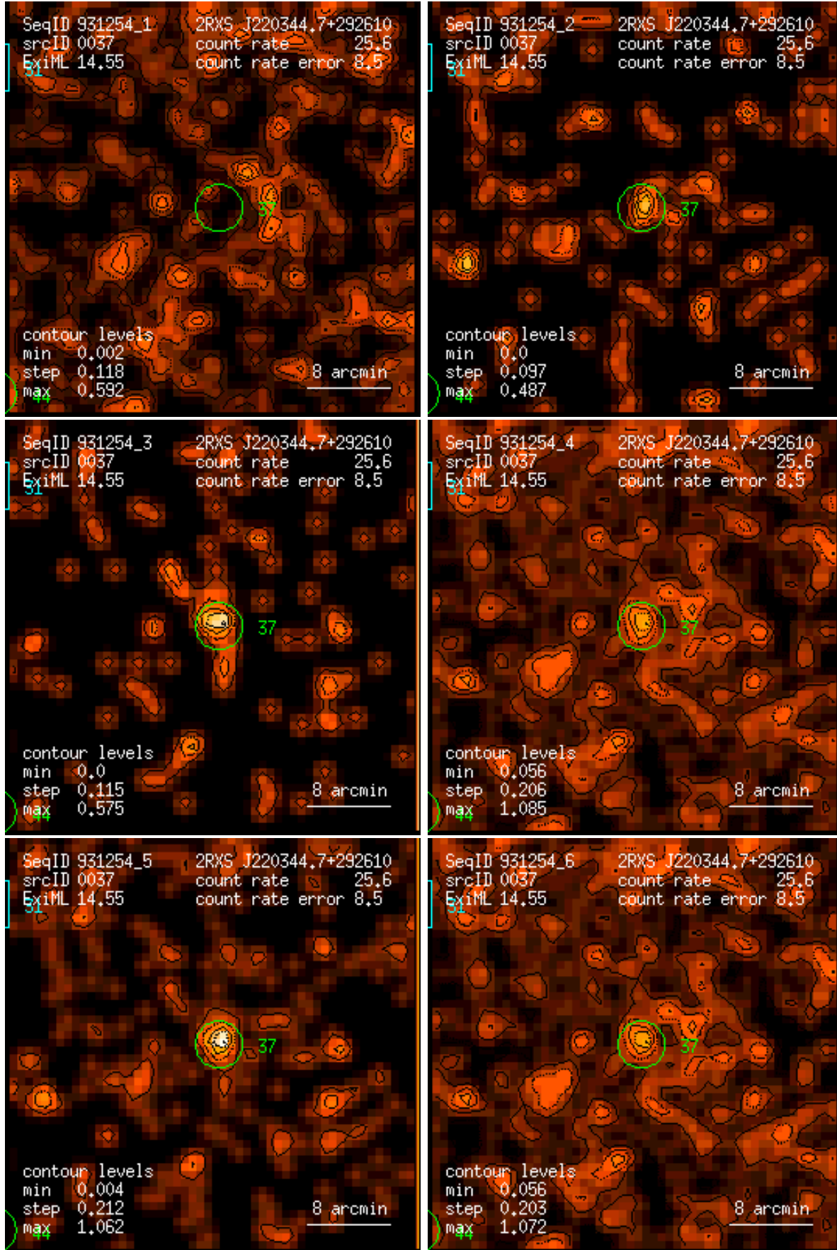
Figure 37: RASS 931254: detection 0037: band rate images, Gaussian filter: (1) PSPC channels 11 – 41, (2) 52 – 90, (3) 91 – 201, (4) 11 – 235, (5) 52 – 201, (6) 11 – 201. Broad band rates in counts/ks. Band rate contour levels in counts/ks/arcmin 2 .
