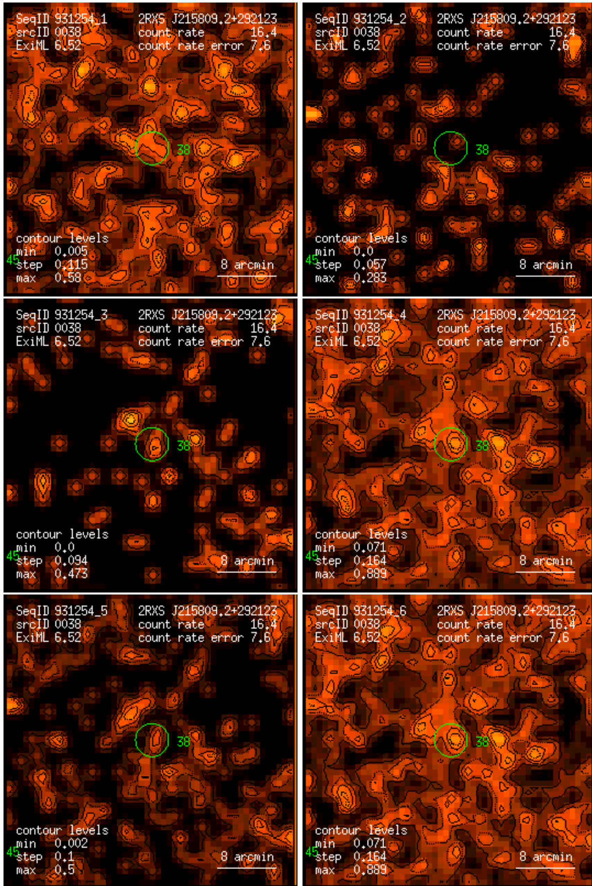
Figure 38: RASS 931254: detection 0038: band rate images, Gaussian filter: (1) PSPC channels 11 – 41, (2) 52 – 90, (3) 91 – 201, (4) 11 – 235, (5) 52 – 201, (6) 11 – 201. Broad band rates in counts/ks. Band rate contour levels in counts/ks/arcmin 2 .
