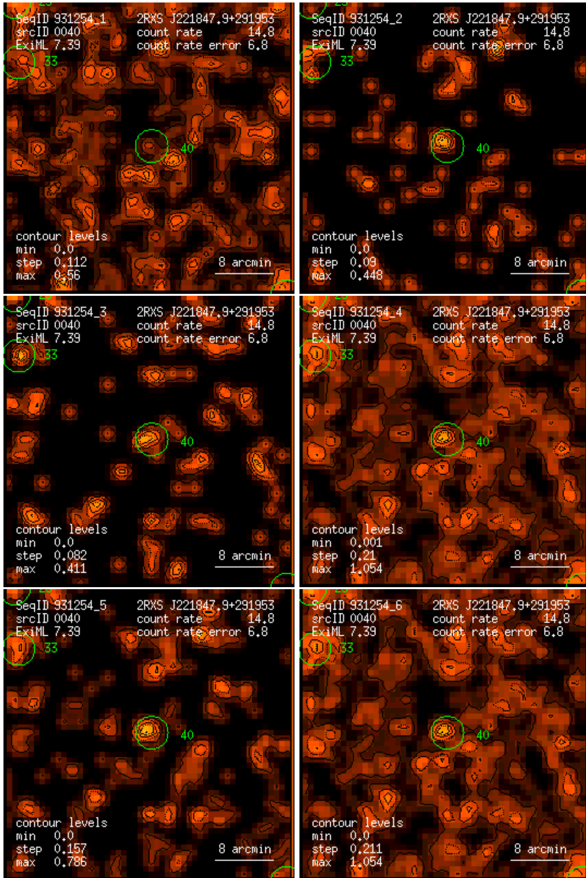
Figure 40: RASS 931254: detection 0040: band rate images, Gaussian filter: (1) PSPC channels 11 – 41, (2) 52 – 90, (3) 91 – 201, (4) 11 – 235, (5) 52 – 201, (6) 11 – 201. Broad band rates in counts/ks. Band rate contour levels in counts/ks/arcmin 2 .
