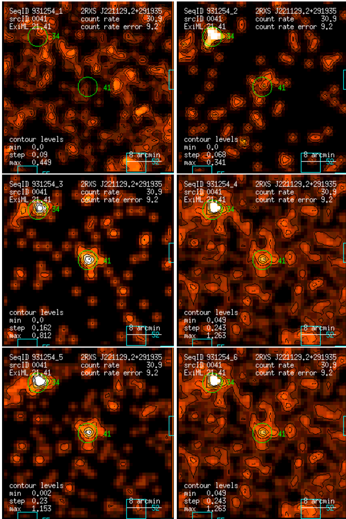
Figure 41: RASS 931254: detection 0041: band rate images, Gaussian filter: (1) PSPC channels 11 – 41, (2) 52 – 90, (3) 91 – 201, (4) 11 – 235, (5) 52 – 201, (6) 11 – 201. Broad band rates in counts/ks. Band rate contour levels in counts/ks/arcmin 2 .
