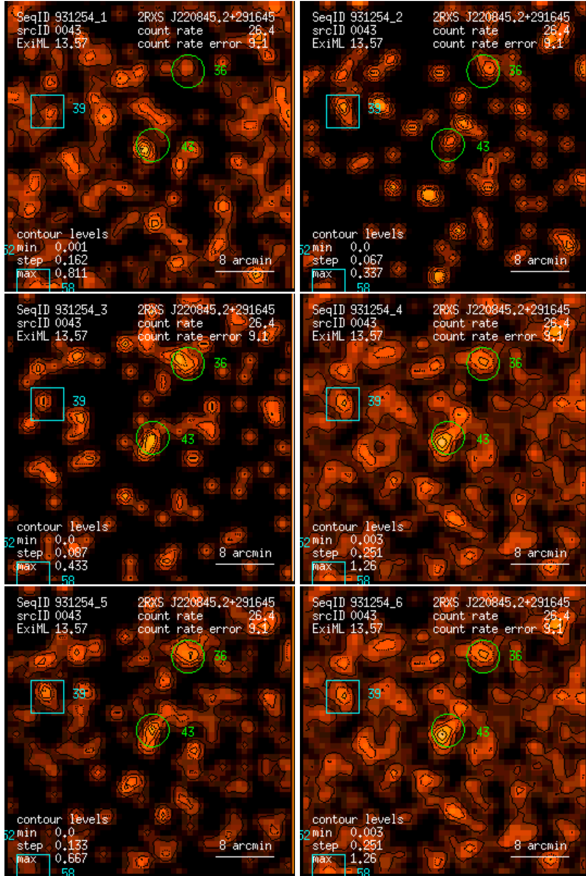
Figure 43: RASS 931254: detection 0043: band rate images, Gaussian filter: (1) PSPC channels 11 – 41, (2) 52 – 90, (3) 91 – 201, (4) 11 – 235, (5) 52 – 201, (6) 11 – 201. Broad band rates in counts/ks. Band rate contour levels in counts/ks/arcmin 2 .
