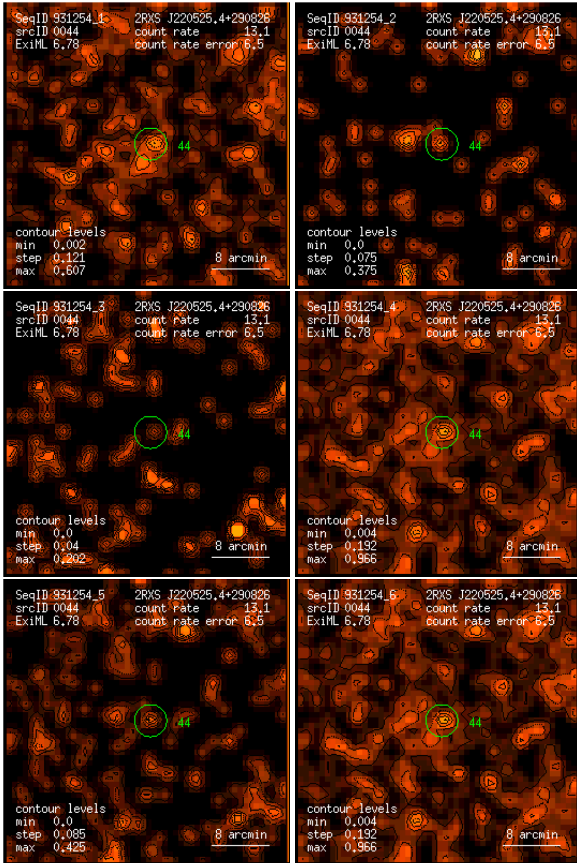
Figure 44: RASS 931254: detection 0044: band rate images, Gaussian filter: (1) PSPC channels 11 – 41, (2) 52 – 90, (3) 91 – 201, (4) 11 – 235, (5) 52 – 201, (6) 11 – 201. Broad band rates in counts/ks. Band rate contour levels in counts/ks/arcmin 2 .
