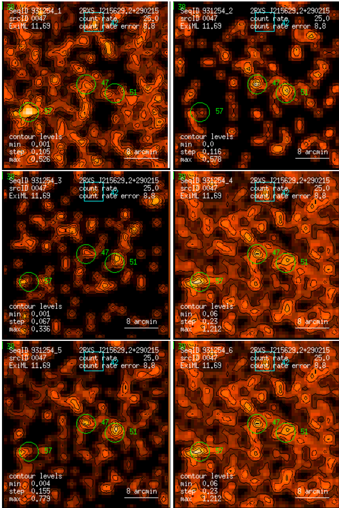
Figure 47: RASS 931254: detection 0047: band rate images, Gaussian filter: (1) PSPC channels 11 – 41, (2) 52 – 90, (3) 91 – 201, (4) 11 – 235, (5) 52 – 201, (6) 11 – 201. Broad band rates in counts/ks. Band rate contour levels in counts/ks/arcmin 2 .
