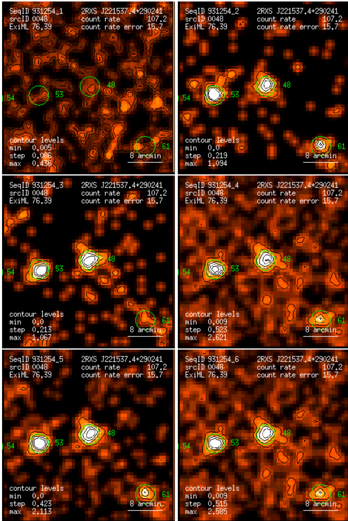
Figure 48: RASS 931254: detection 0048: band rate images, Gaussian filter: (1) PSPC channels 11 – 41, (2) 52 – 90, (3) 91 – 201, (4) 11 – 235, (5) 52 – 201, (6) 11 – 201. Broad band rates in counts/ks. Band rate contour levels in counts/ks/arcmin 2 .
