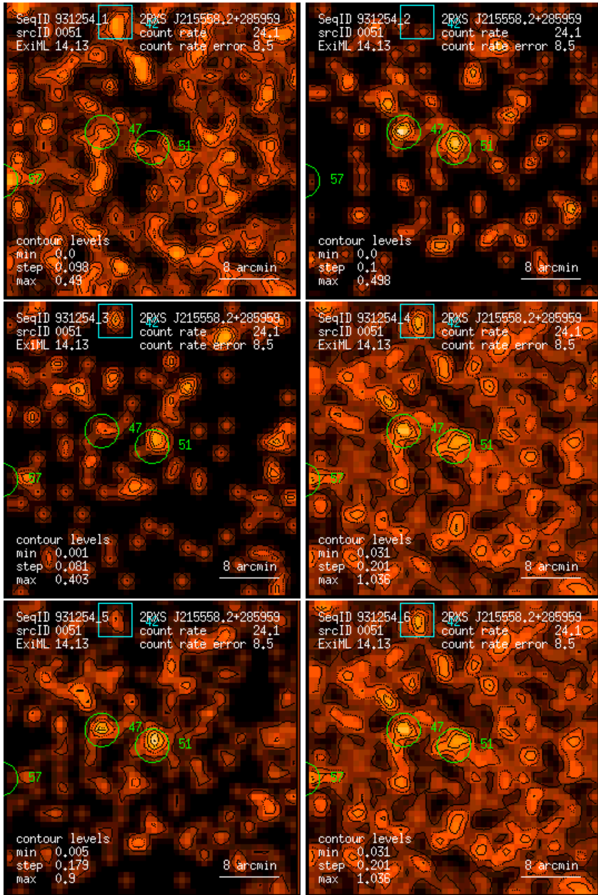
Figure 51: RASS 931254: detection 0051: band rate images, Gaussian filter: (1) PSPC channels 11 – 41, (2) 52 – 90, (3) 91 – 201, (4) 11 – 235, (5) 52 – 201, (6) 11 – 201. Broad band rates in counts/ks. Band rate contour levels in counts/ks/arcmin 2 .
