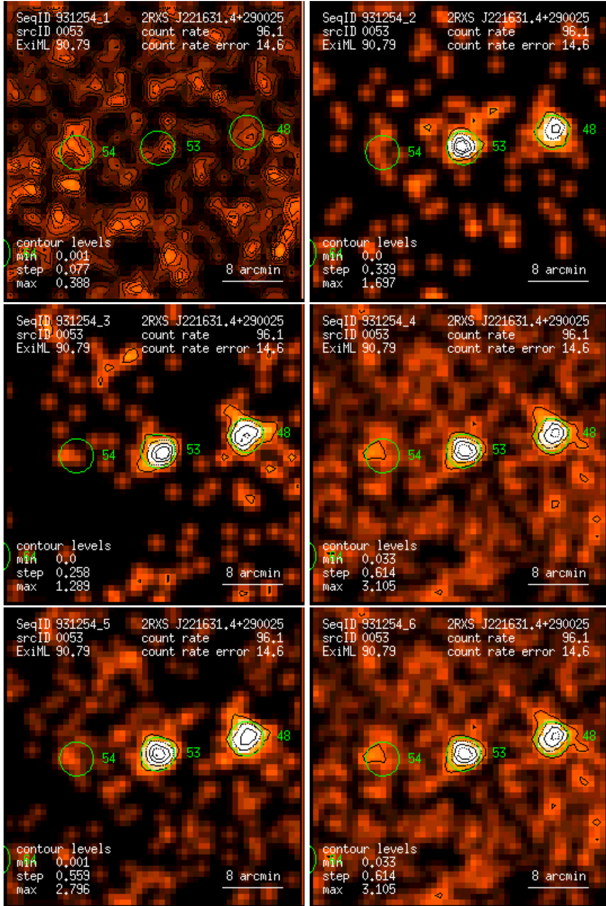
Figure 53: RASS 931254: detection 0053: band rate images, Gaussian filter: (1) PSPC channels 11 – 41, (2) 52 – 90, (3) 91 – 201, (4) 11 – 235, (5) 52 – 201, (6) 11 – 201. Broad band rates in counts/ks. Band rate contour levels in counts/ks/arcmin 2 .
