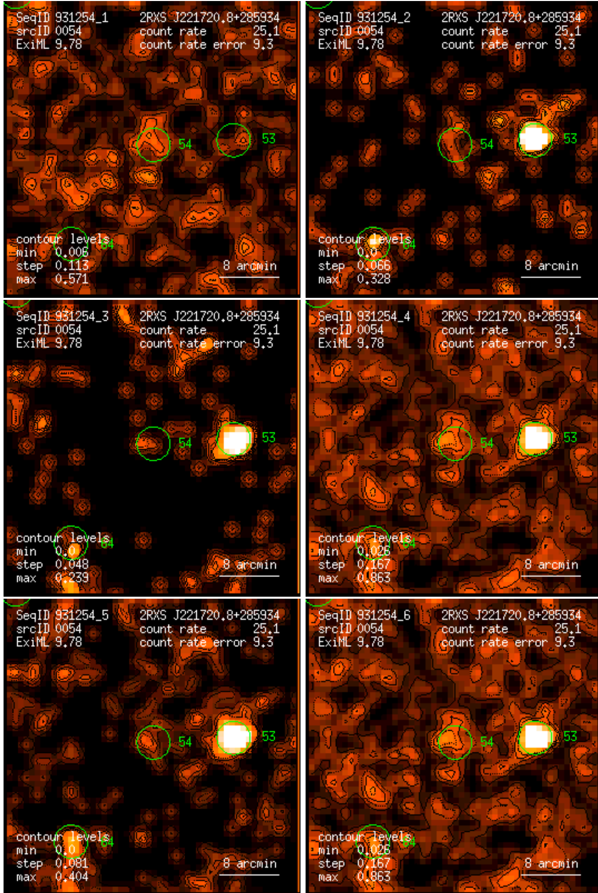
Figure 54: RASS 931254: detection 0054: band rate images, Gaussian filter: (1) PSPC channels 11 – 41, (2) 52 – 90, (3) 91 – 201, (4) 11 – 235, (5) 52 – 201, (6) 11 – 201. Broad band rates in counts/ks. Band rate contour levels in counts/ks/arcmin 2 .
