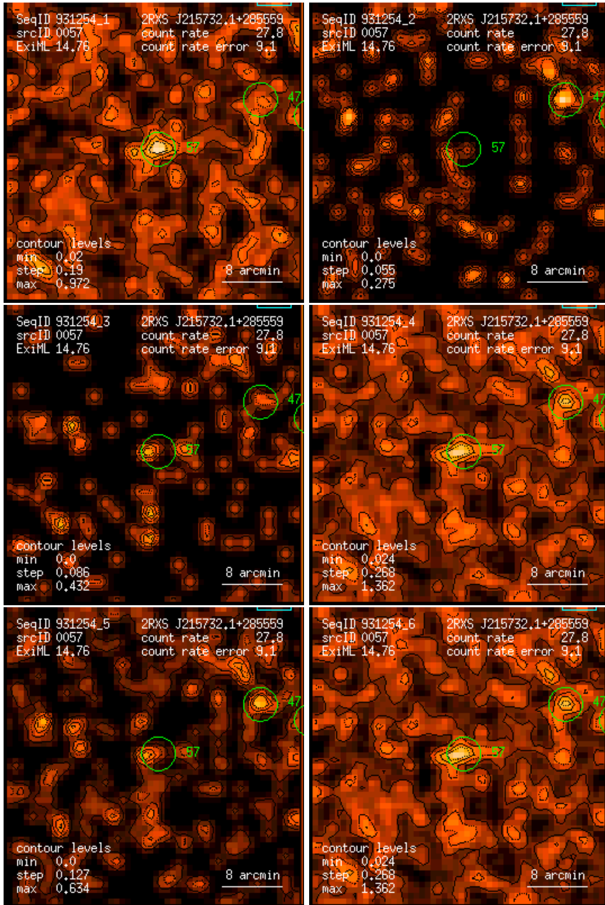
Figure 57: RASS 931254: detection 0057: band rate images, Gaussian filter: (1) PSPC channels 11 – 41, (2) 52 – 90, (3) 91 – 201, (4) 11 – 235, (5) 52 – 201, (6) 11 – 201. Broad band rates in counts/ks. Band rate contour levels in counts/ks/arcmin 2 .
