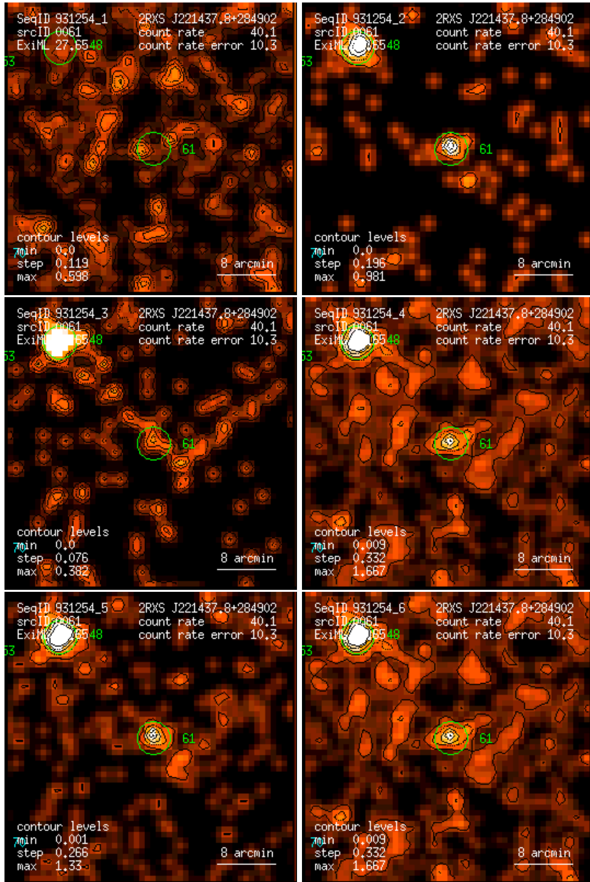
Figure 61: RASS 931254: detection 0061: band rate images, Gaussian filter: (1) PSPC channels 11 – 41, (2) 52 – 90, (3) 91 – 201, (4) 11 – 235, (5) 52 – 201, (6) 11 – 201. Broad band rates in counts/ks. Band rate contour levels in counts/ks/arcmin 2 .
