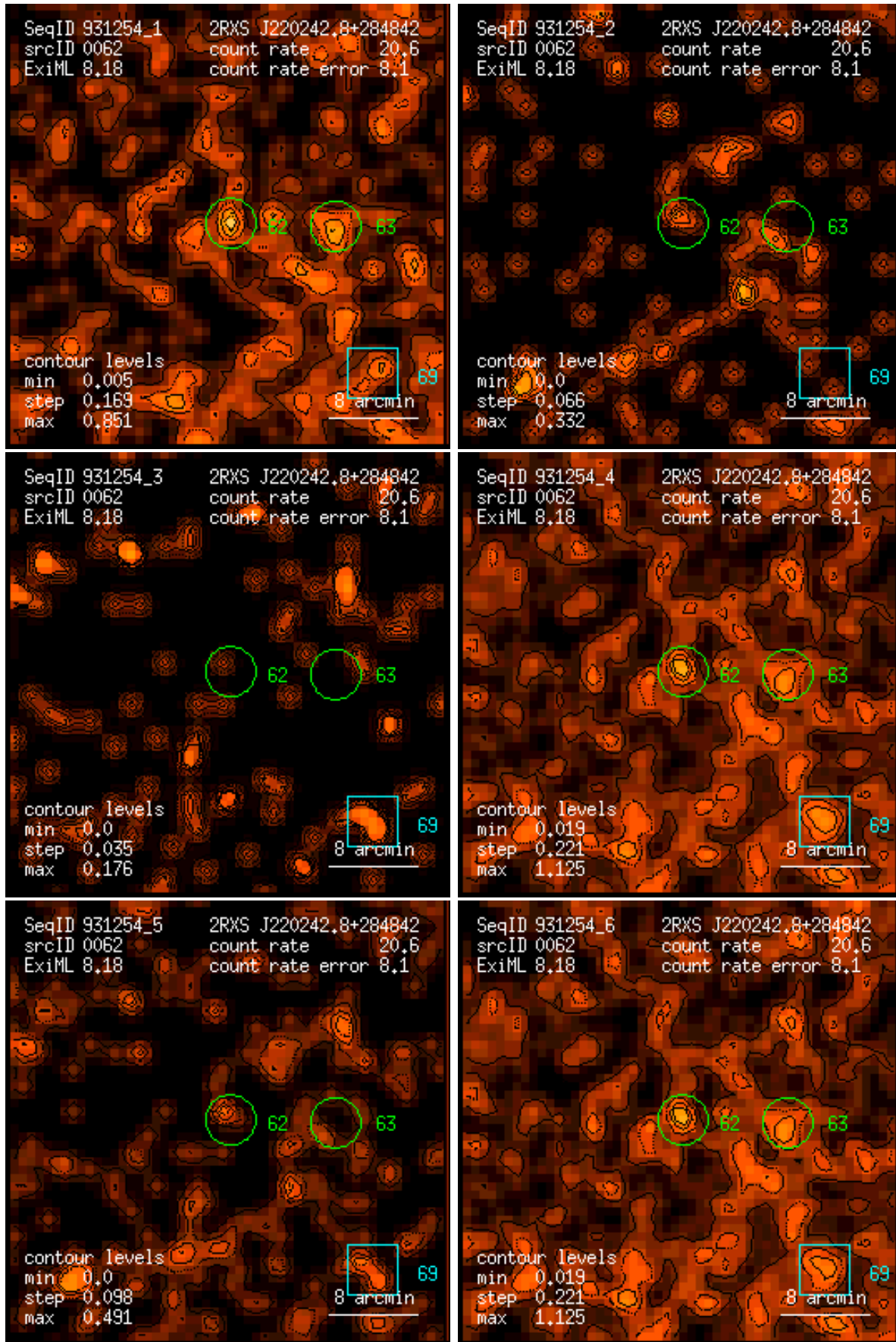
Figure 62: RASS 931254: detection 0062: band rate images, Gaussian filter: (1) PSPC channels 11 – 41, (2) 52 – 90, (3) 91 – 201, (4) 11 – 235, (5) 52 – 201, (6) 11 – 201. Broad band rates in counts/ks. Band rate contour levels in counts/ks/arcmin 2 .
