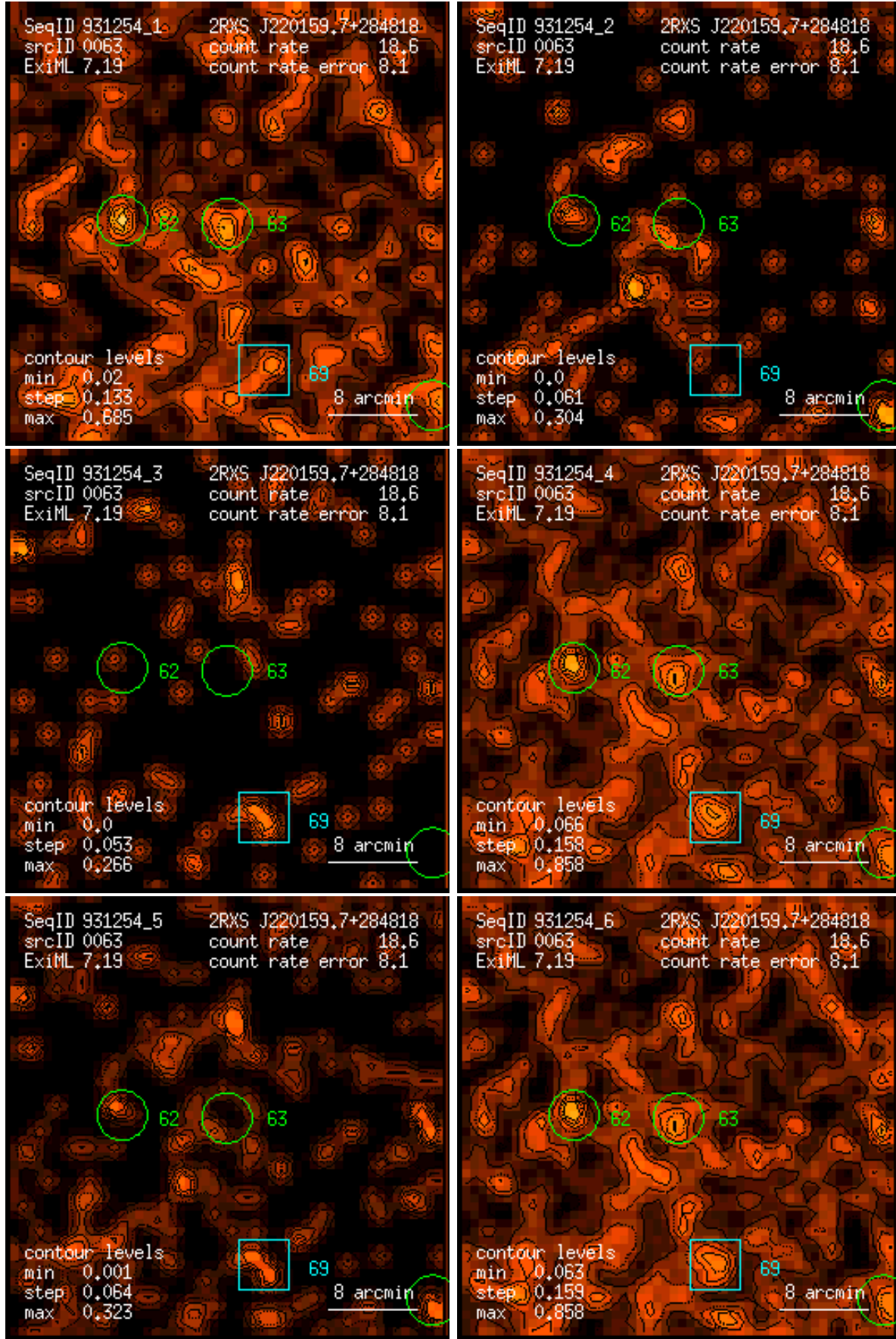
Figure 63: RASS 931254: detection 0063: band rate images, Gaussian filter: (1) PSPC channels 11 – 41, (2) 52 – 90, (3) 91 – 201, (4) 11 – 235, (5) 52 – 201, (6) 11 – 201. Broad band rates in counts/ks. Band rate contour levels in counts/ks/arcmin 2 .
