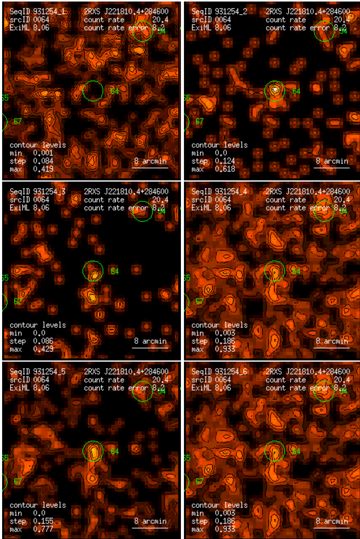
Figure 64: RASS 931254: detection 0064: band rate images, Gaussian filter: (1) PSPC channels 11 – 41, (2) 52 – 90, (3) 91 – 201, (4) 11 – 235, (5) 52 – 201, (6) 11 – 201. Broad band rates in counts/ks. Band rate contour levels in counts/ks/arcmin 2 .
