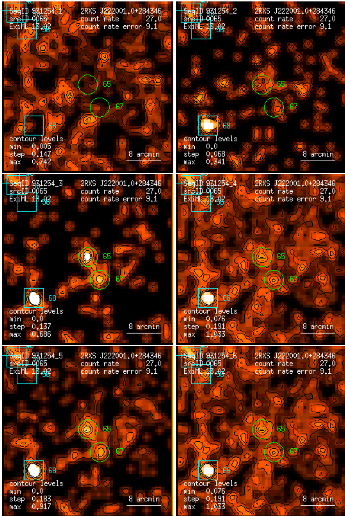
Figure 65: RASS 931254: detection 0065: band rate images, Gaussian filter: (1) PSPC channels 11 – 41, (2) 52 – 90, (3) 91 – 201, (4) 11 – 235, (5) 52 – 201, (6) 11 – 201. Broad band rates in counts/ks. Band rate contour levels in counts/ks/arcmin 2 .
