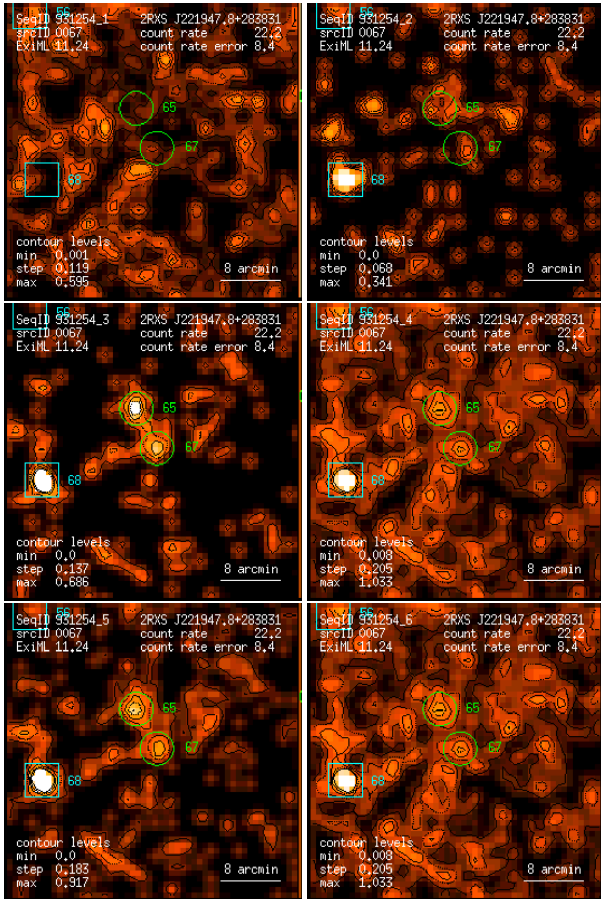
Figure 67: RASS 931254: detection 0067: band rate images, Gaussian filter: (1) PSPC channels 11 – 41, (2) 52 – 90, (3) 91 – 201, (4) 11 – 235, (5) 52 – 201, (6) 11 – 201. Broad band rates in counts/ks. Band rate contour levels in counts/ks/arcmin 2 .
