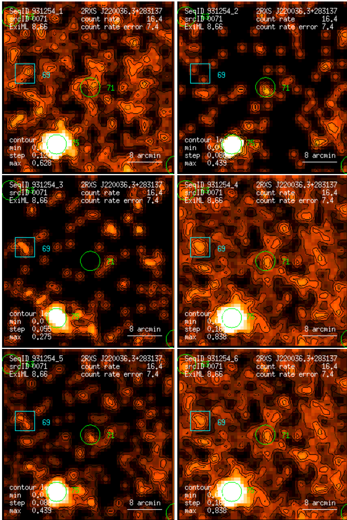
Figure 71: RASS 931254: detection 0071: band rate images, Gaussian filter: (1) PSPC channels 11 – 41, (2) 52 – 90, (3) 91 – 201, (4) 11 – 235, (5) 52 – 201, (6) 11 – 201. Broad band rates in counts/ks. Band rate contour levels in counts/ks/arcmin 2 .
