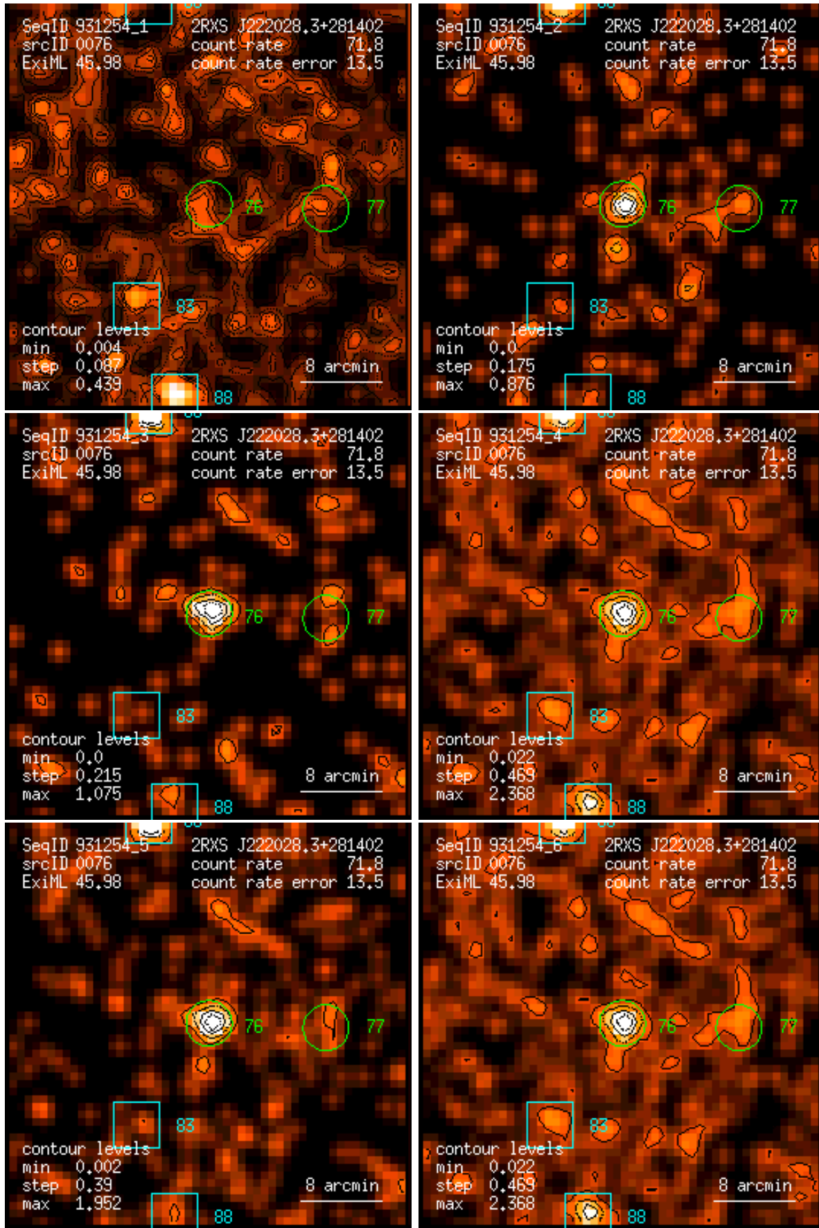
Figure 76: RASS 931254: detection 0076: band rate images, Gaussian filter: (1) PSPC channels 11 – 41, (2) 52 – 90, (3) 91 – 201, (4) 11 – 235, (5) 52 – 201, (6) 11 – 201. Broad band rates in counts/ks. Band rate contour levels in counts/ks/arcmin 2 .
