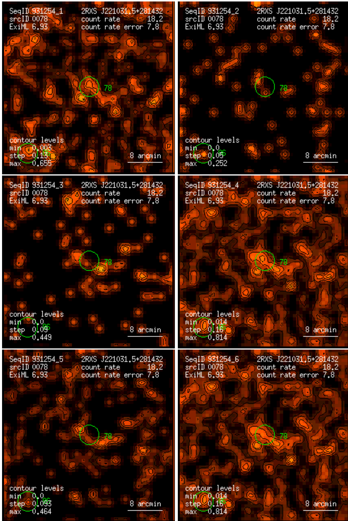
Figure 78: RASS 931254: detection 0078: band rate images, Gaussian filter: (1) PSPC channels 11 – 41, (2) 52 – 90, (3) 91 – 201, (4) 11 – 235, (5) 52 – 201, (6) 11 – 201. Broad band rates in counts/ks. Band rate contour levels in counts/ks/arcmin 2 .
