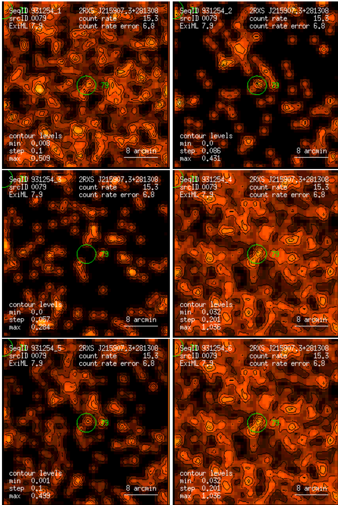
Figure 79: RASS 931254: detection 0079: band rate images, Gaussian filter: (1) PSPC channels 11 – 41, (2) 52 – 90, (3) 91 – 201, (4) 11 – 235, (5) 52 – 201, (6) 11 – 201. Broad band rates in counts/ks. Band rate contour levels in counts/ks/arcmin 2 .
