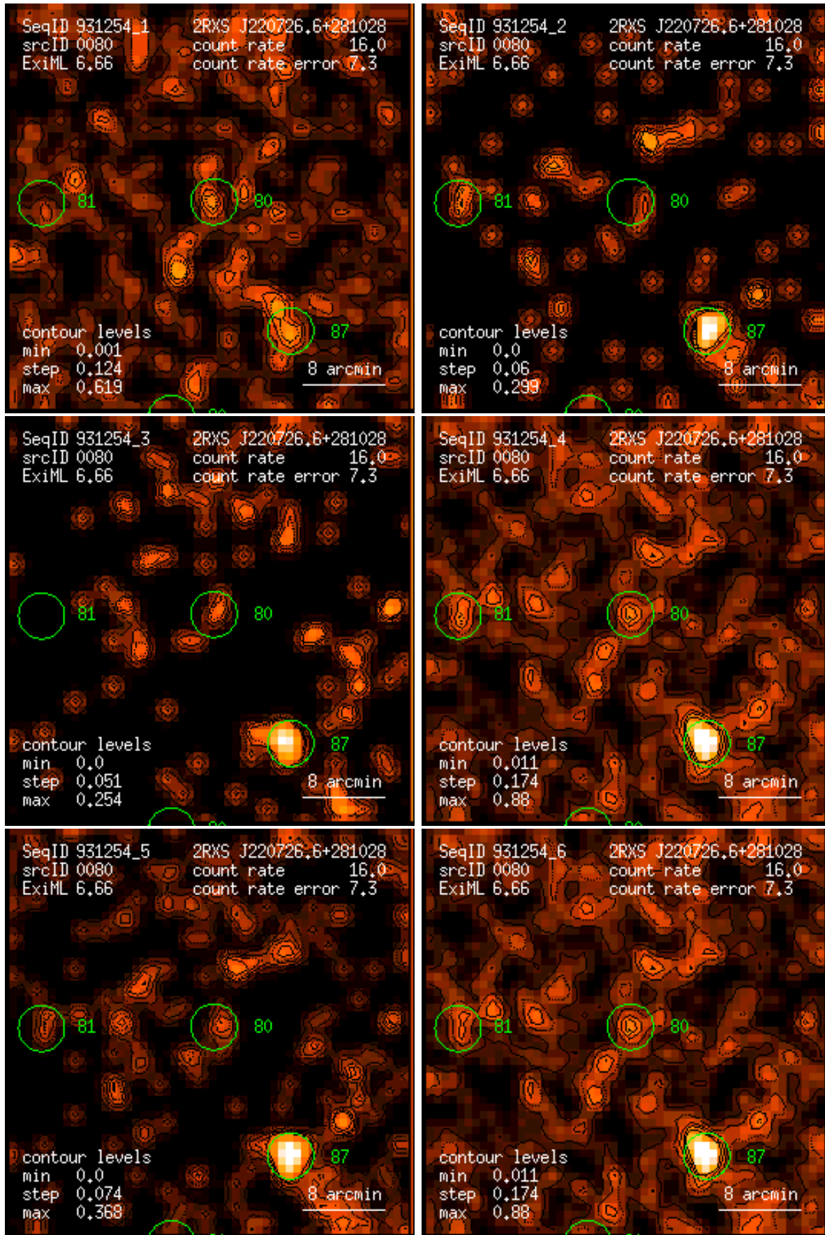
Figure 80: RASS 931254: detection 0080: band rate images, Gaussian filter: (1) PSPC channels 11 – 41, (2) 52 – 90, (3) 91 – 201, (4) 11 – 235, (5) 52 – 201, (6) 11 – 201. Broad band rates in counts/ks. Band rate contour levels in counts/ks/arcmin 2 .
