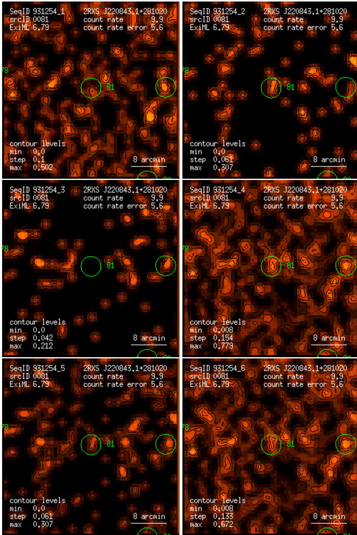
Figure 81: RASS 931254: detection 0081: band rate images, Gaussian filter: (1) PSPC channels 11 – 41, (2) 52 – 90, (3) 91 – 201, (4) 11 – 235, (5) 52 – 201, (6) 11 – 201. Broad band rates in counts/ks. Band rate contour levels in counts/ks/arcmin 2 .
