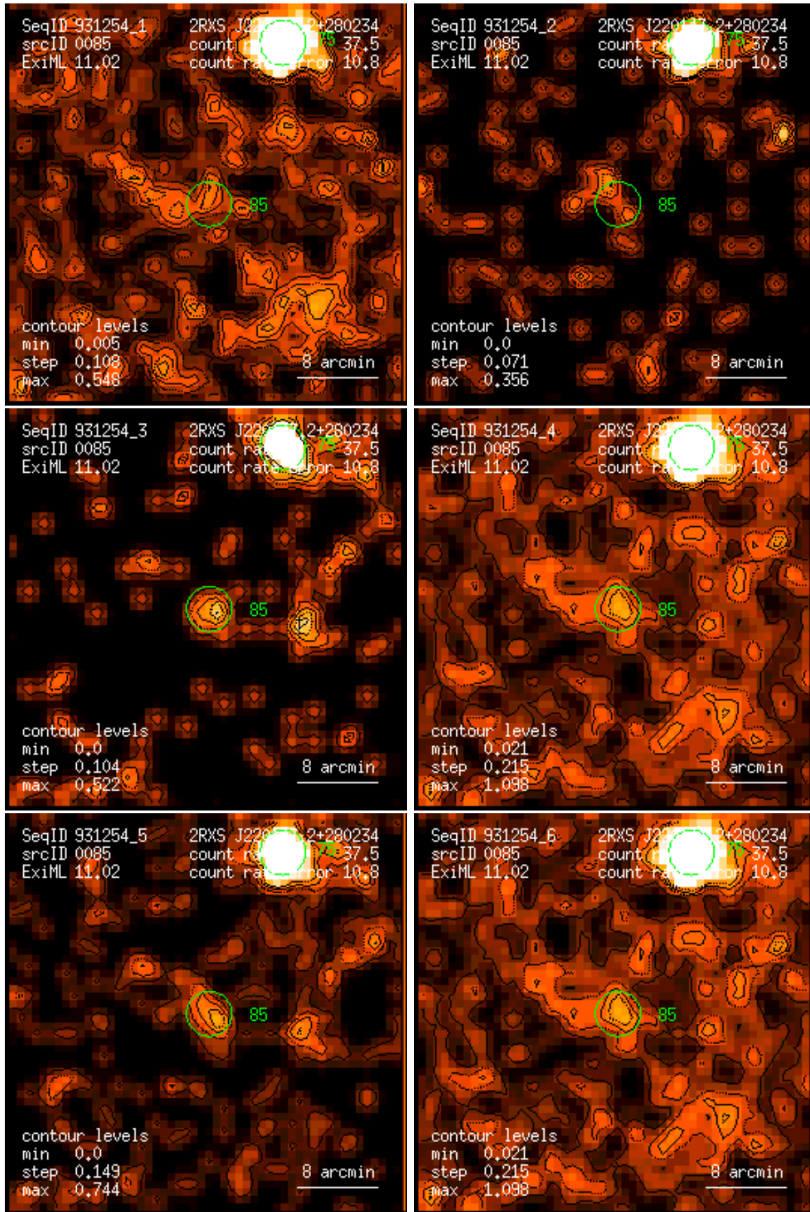
Figure 85: RASS 931254: detection 0085: band rate images, Gaussian filter: (1) PSPC channels 11 – 41, (2) 52 – 90, (3) 91 – 201, (4) 11 – 235, (5) 52 – 201, (6) 11 – 201. Broad band rates in counts/ks. Band rate contour levels in counts/ks/arcmin 2 .
