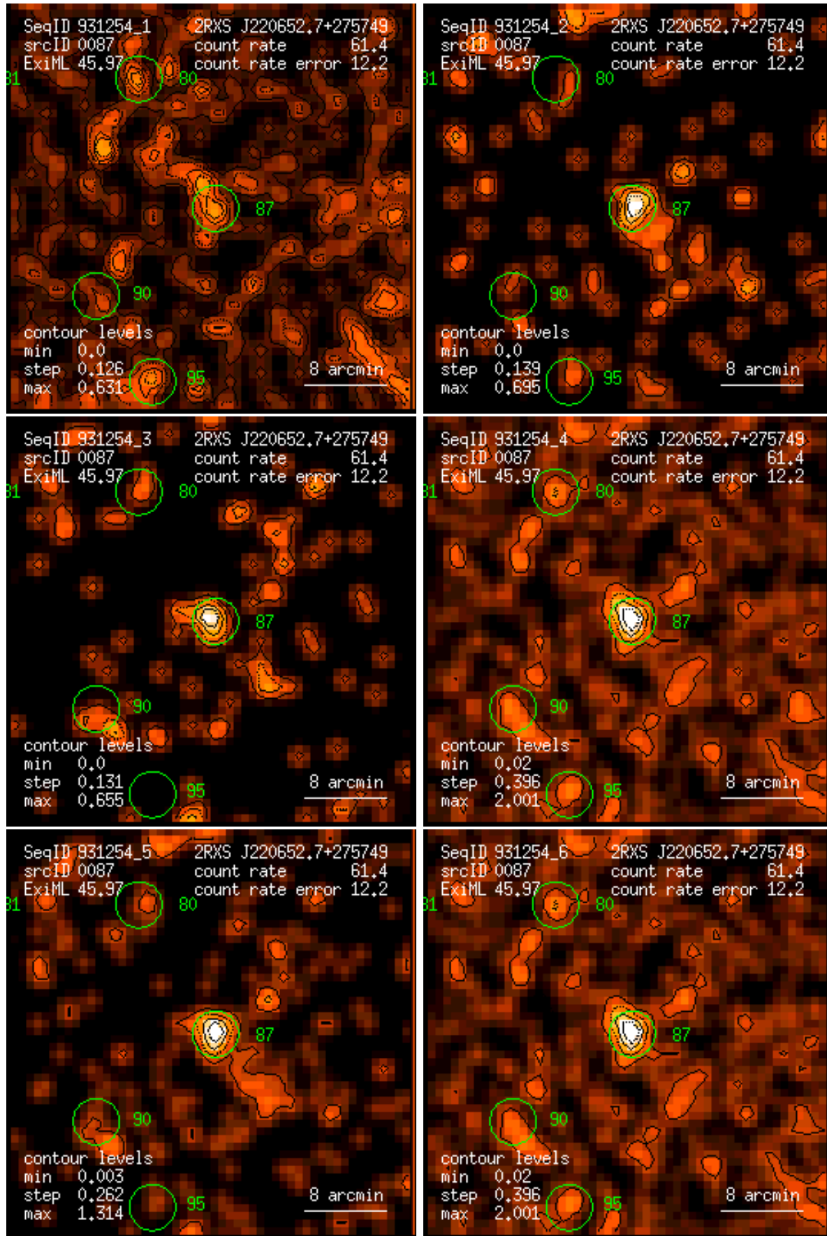
Figure 87: RASS 931254: detection 0087: band rate images, Gaussian filter: (1) PSPC channels 11 – 41, (2) 52 – 90, (3) 91 – 201, (4) 11 – 235, (5) 52 – 201, (6) 11 – 201. Broad band rates in counts/ks. Band rate contour levels in counts/ks/arcmin 2 .
