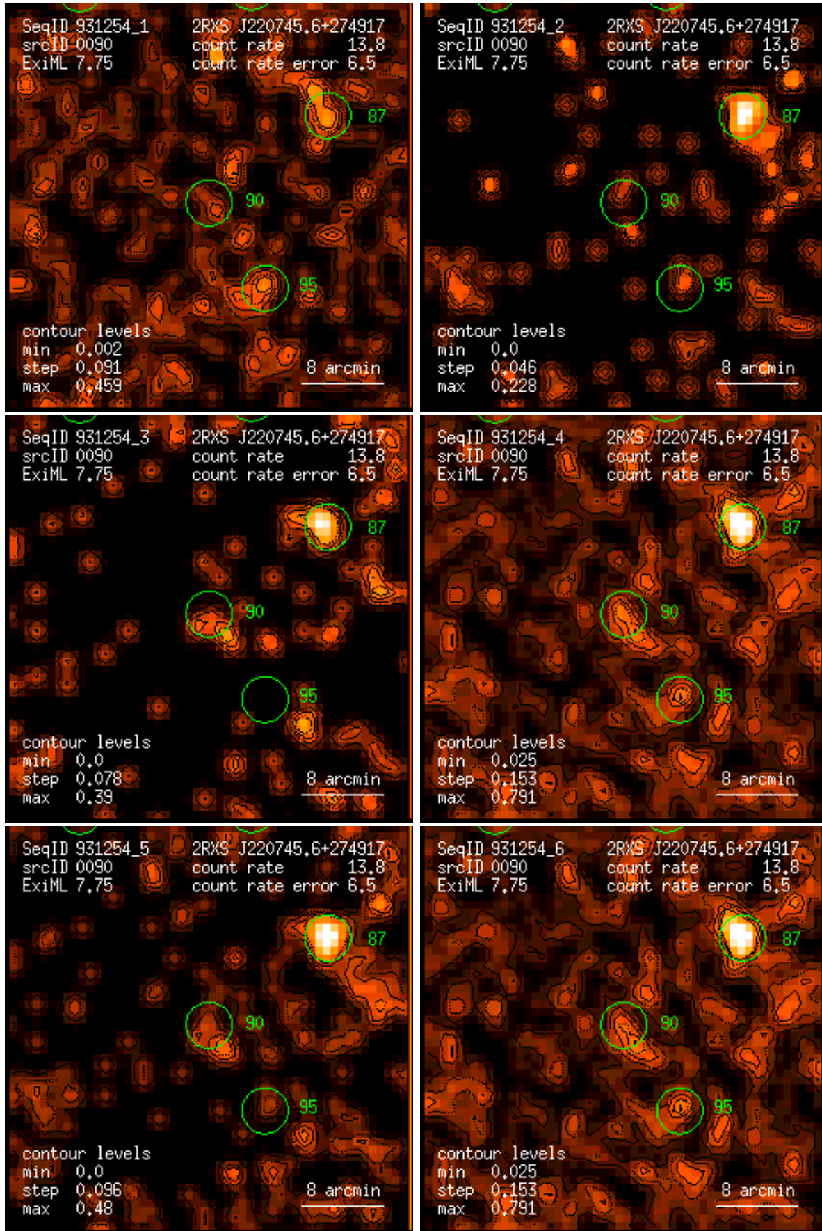
Figure 90: RASS 931254: detection 0090: band rate images, Gaussian filter: (1) PSPC channels 11 – 41, (2) 52 – 90, (3) 91 – 201, (4) 11 – 235, (5) 52 – 201, (6) 11 – 201. Broad band rates in counts/ks. Band rate contour levels in counts/ks/arcmin 2 .
