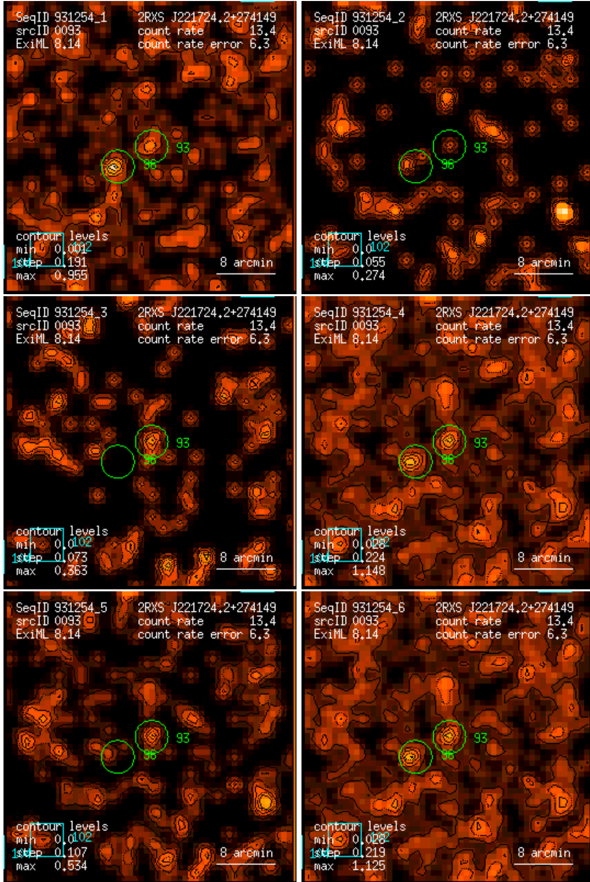
Figure 93: RASS 931254: detection 0093: band rate images, Gaussian filter: (1) PSPC channels 11 – 41, (2) 52 – 90, (3) 91 – 201, (4) 11 – 235, (5) 52 – 201, (6) 11 – 201. Broad band rates in counts/ks. Band rate contour levels in counts/ks/arcmin 2 .
