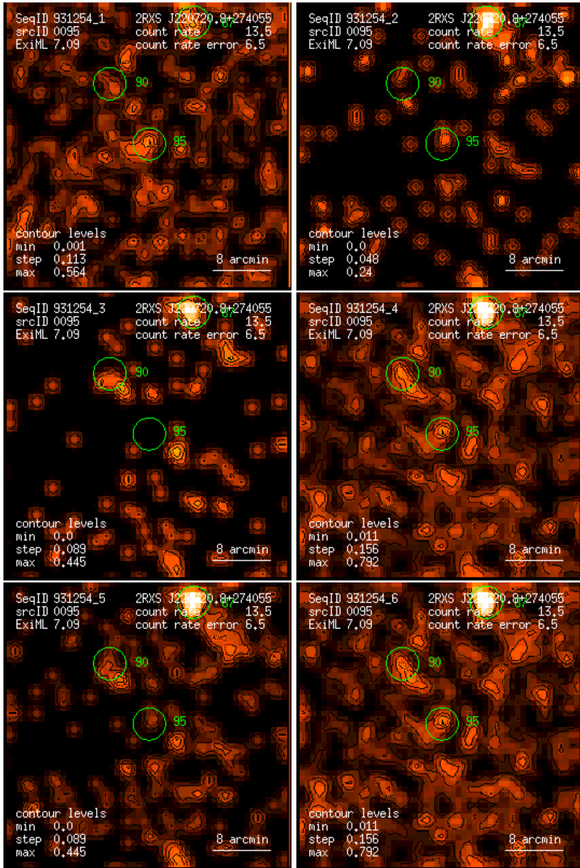
Figure 95: RASS 931254: detection 0095: band rate images, Gaussian filter: (1) PSPC channels 11 – 41, (2) 52 – 90, (3) 91 – 201, (4) 11 – 235, (5) 52 – 201, (6) 11 – 201. Broad band rates in counts/ks. Band rate contour levels in counts/ks/arcmin 2 .
