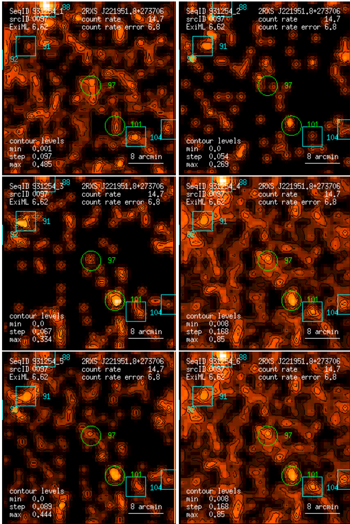
Figure 97: RASS 931254: detection 0097: band rate images, Gaussian filter: (1) PSPC channels 11 – 41, (2) 52 – 90, (3) 91 – 201, (4) 11 – 235, (5) 52 – 201, (6) 11 – 201. Broad band rates in counts/ks. Band rate contour levels in counts/ks/arcmin 2 .
