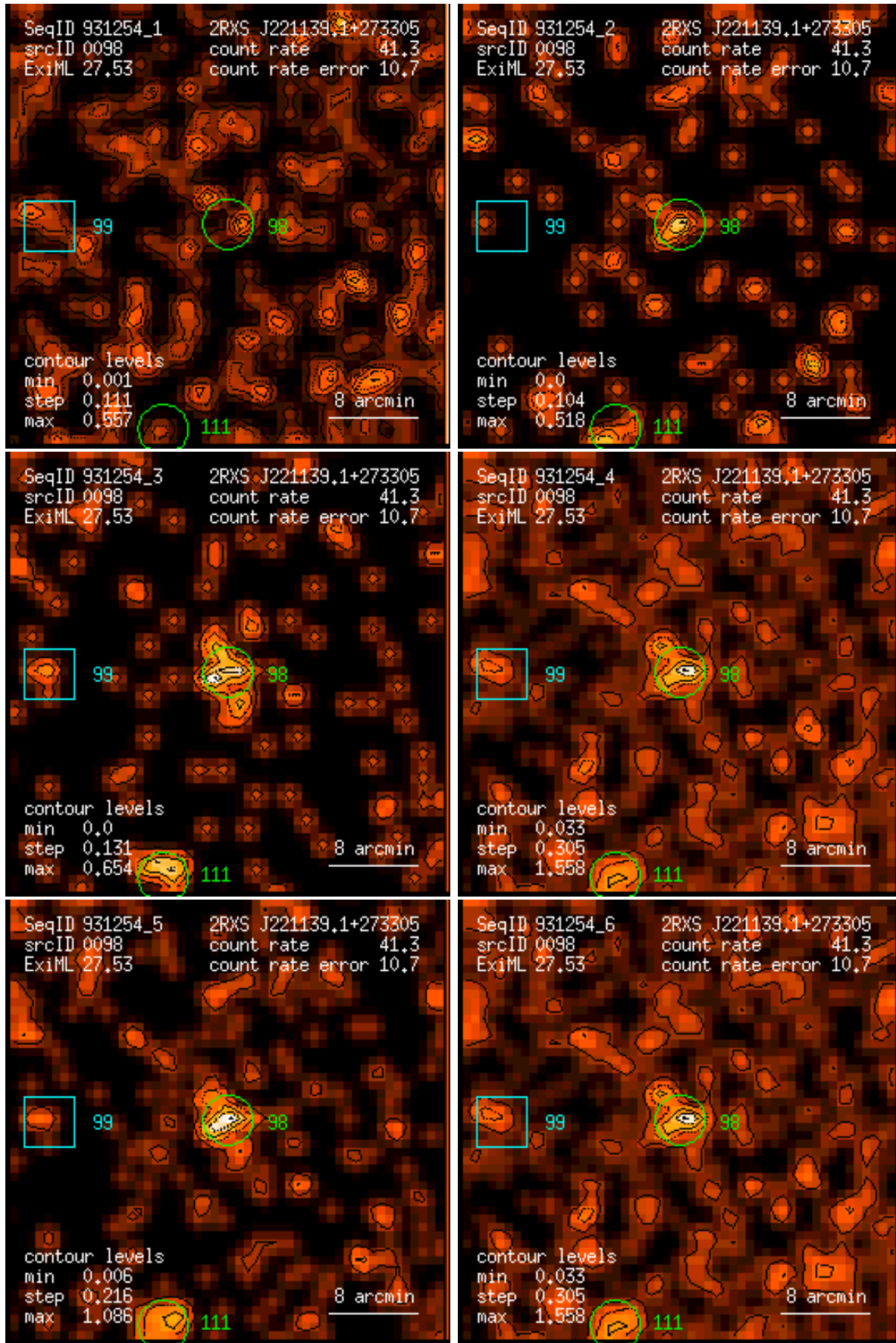
Figure 98: RASS 931254: detection 0098: band rate images, Gaussian filter: (1) PSPC channels 11 – 41, (2) 52 – 90, (3) 91 – 201, (4) 11 – 235, (5) 52 – 201, (6) 11 – 201. Broad band rates in counts/ks. Band rate contour levels in counts/ks/arcmin 2 .
