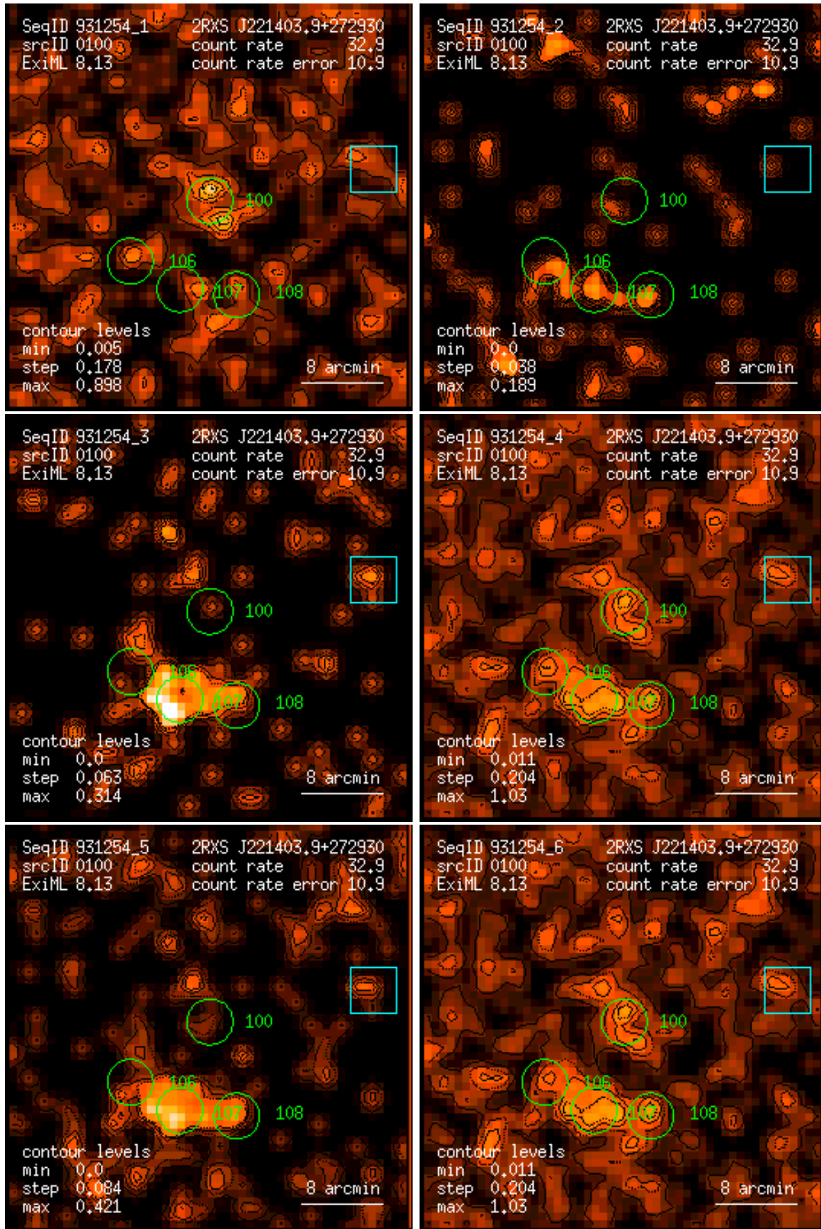
Figure 100: RASS 931254: detection 0100: band rate images, Gaussian filter: (1) PSPC channels 11 – 41, (2) 52 – 90, (3) 91 – 201, (4) 11 – 235, (5) 52 – 201, (6) 11 – 201. Broad band rates in counts/ks. Band rate contour levels in counts/ks/arcmin 2 .
