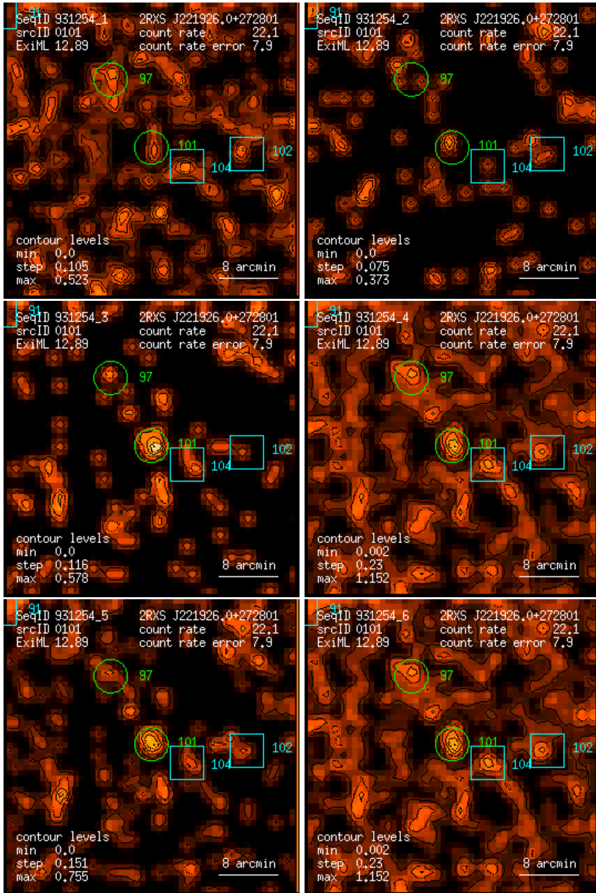
Figure 101: RASS 931254: detection 0101: band rate images, Gaussian filter: (1) PSPC channels 11 – 41, (2) 52 – 90, (3) 91 – 201, (4) 11 – 235, (5) 52 – 201, (6) 11 – 201. Broad band rates in counts/ks. Band rate contour levels in counts/ks/arcmin 2 .
