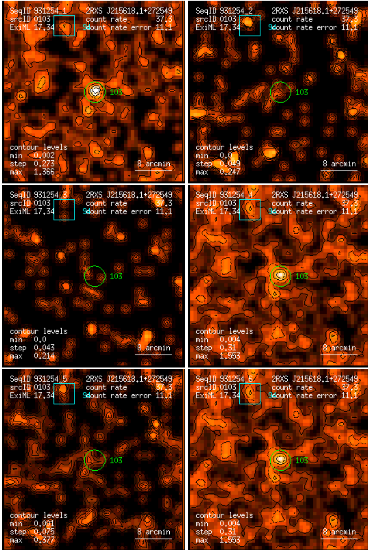
Figure 103: RASS 931254: detection 0103: band rate images, Gaussian filter: (1) PSPC channels 11 – 41, (2) 52 – 90, (3) 91 – 201, (4) 11 – 235, (5) 52 – 201, (6) 11 – 201. Broad band rates in counts/ks. Band rate contour levels in counts/ks/arcmin 2 .
