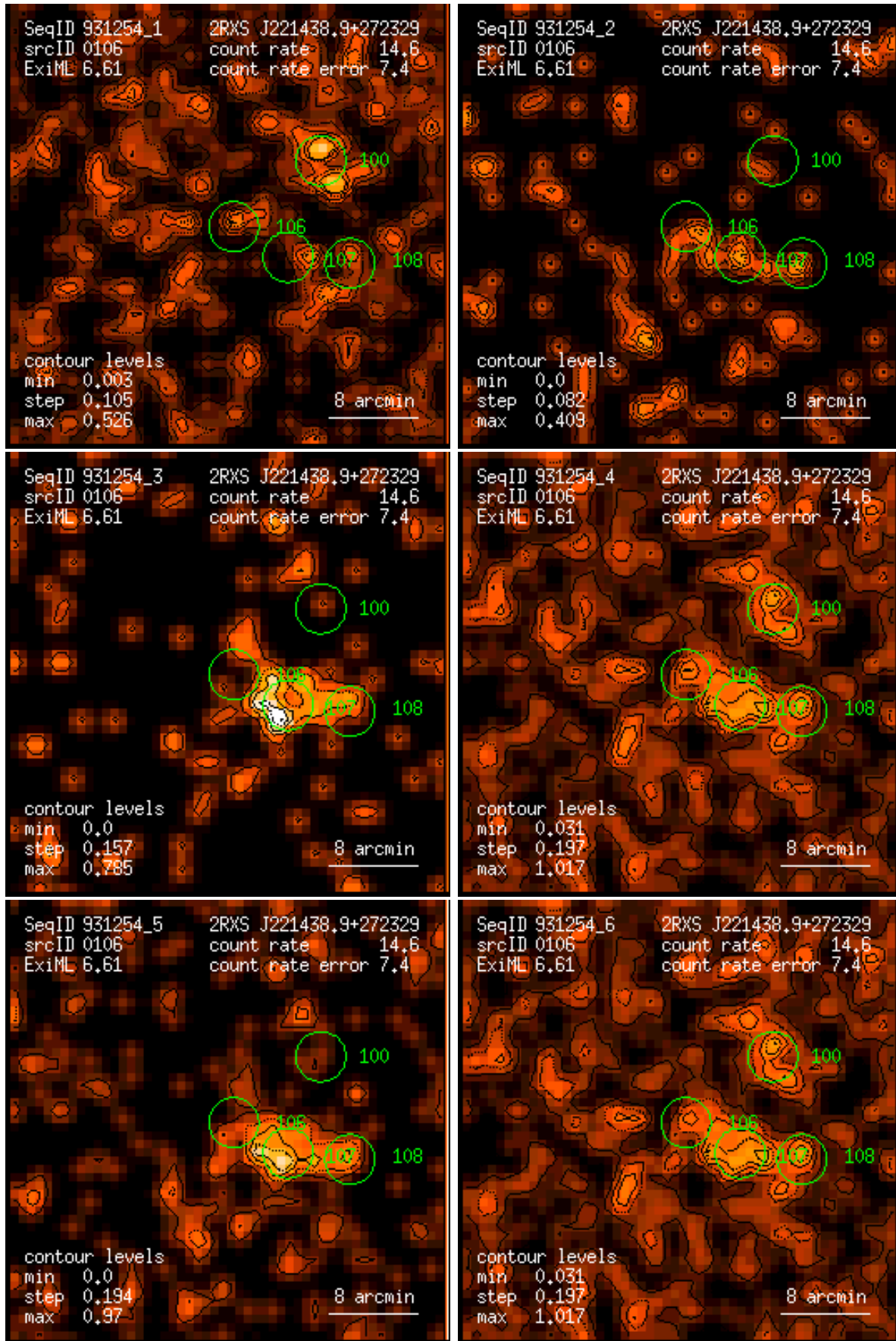
Figure 106: RASS 931254: detection 0106: band rate images, Gaussian filter: (1) PSPC channels 11 – 41, (2) 52 – 90, (3) 91 – 201, (4) 11 – 235, (5) 52 – 201, (6) 11 – 201. Broad band rates in counts/ks. Band rate contour levels in counts/ks/arcmin 2 .
