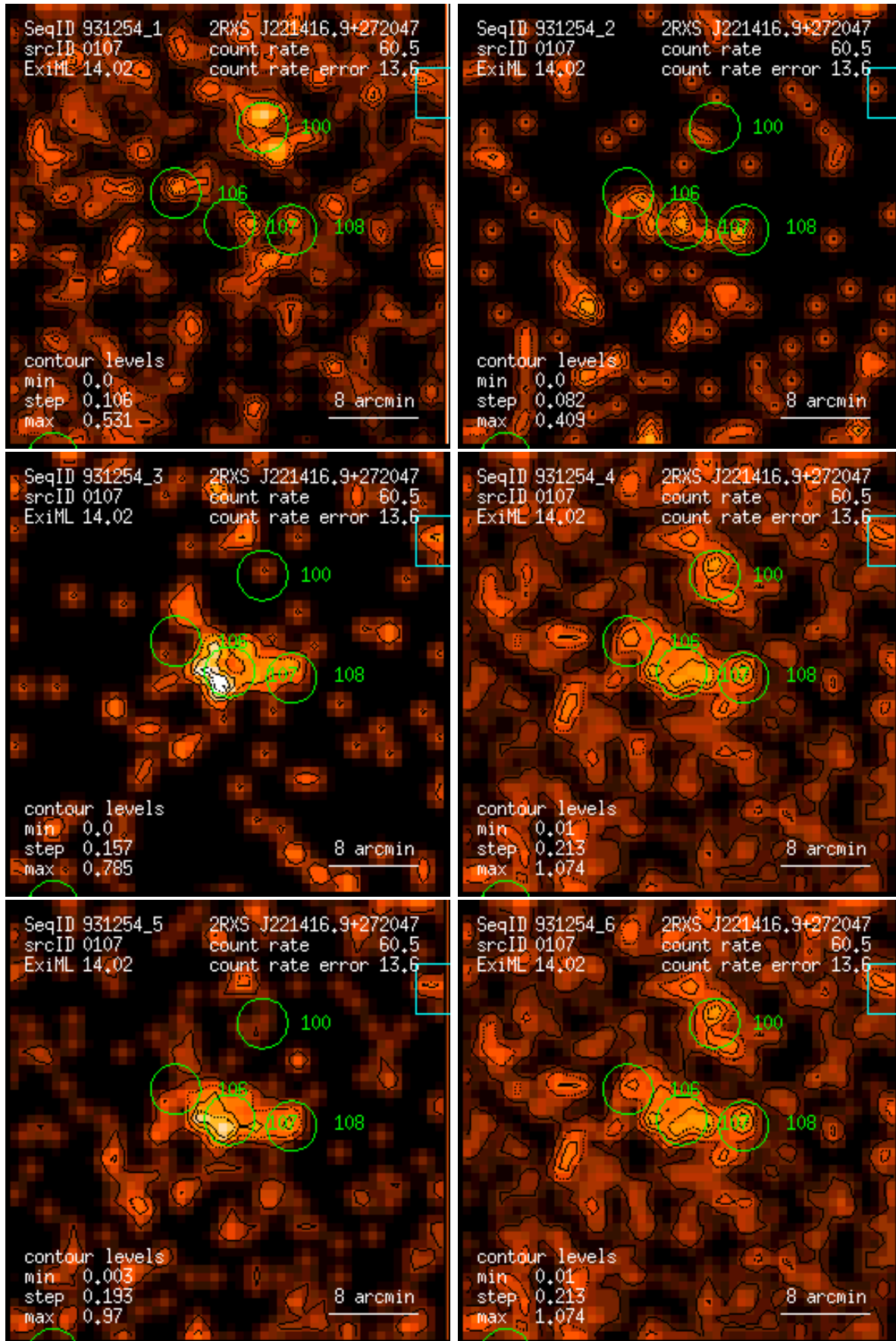
Figure 107: RASS 931254: detection 0107: band rate images, Gaussian filter: (1) PSPC channels 11 – 41, (2) 52 – 90, (3) 91 – 201, (4) 11 – 235, (5) 52 – 201, (6) 11 – 201. Broad band rates in counts/ks. Band rate contour levels in counts/ks/arcmin 2 .
