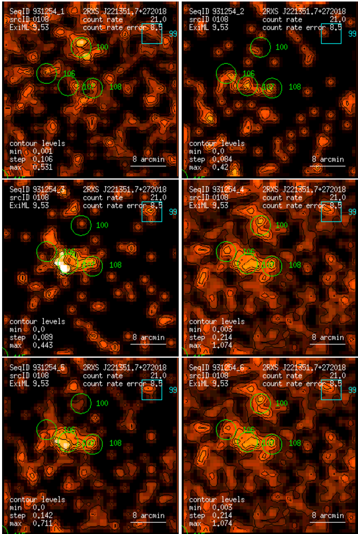
Figure 108: RASS 931254: detection 0108: band rate images, Gaussian filter: (1) PSPC channels 11 – 41, (2) 52 – 90, (3) 91 – 201, (4) 11 – 235, (5) 52 – 201, (6) 11 – 201. Broad band rates in counts/ks. Band rate contour levels in counts/ks/arcmin 2 .
