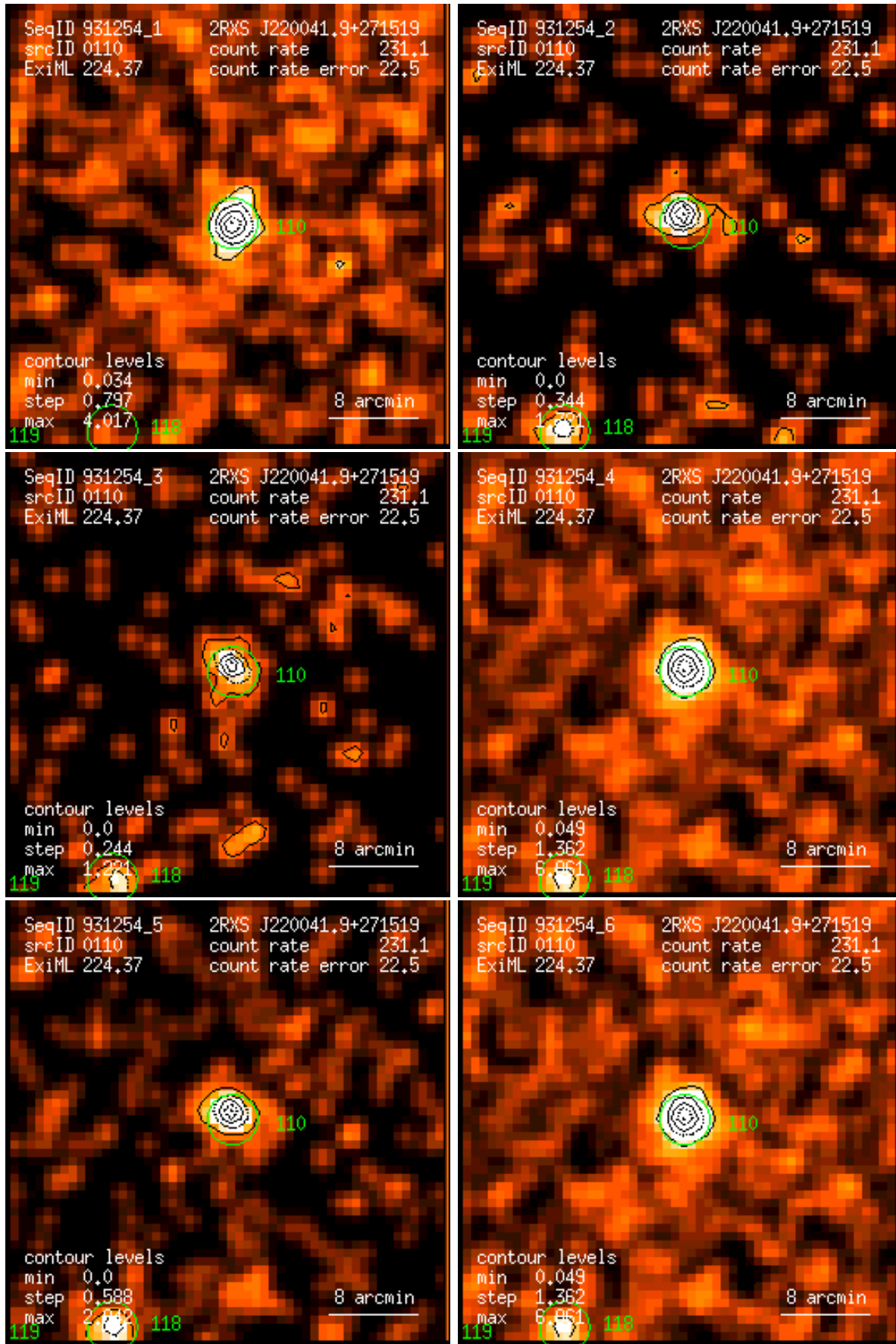
Figure 110: RASS 931254: detection 0110: band rate images, Gaussian filter: (1) PSPC channels 11 – 41, (2) 52 – 90, (3) 91 – 201, (4) 11 – 235, (5) 52 – 201, (6) 11 – 201. Broad band rates in counts/ks. Band rate contour levels in counts/ks/arcmin 2 .
